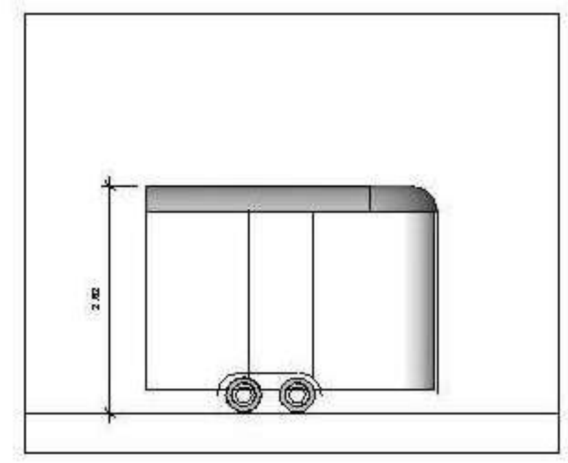
4 Cabin West Elevation 1:50
