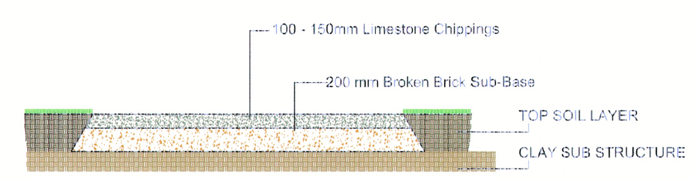
CROSS - SECTION OF TRACK
