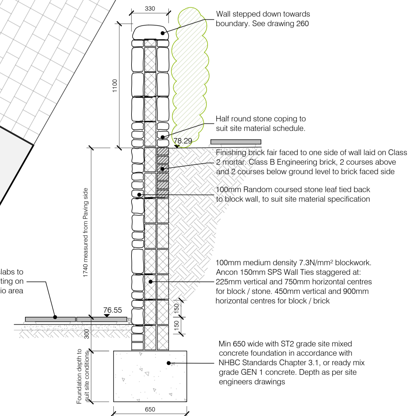
RETAINING WALL 1:20
