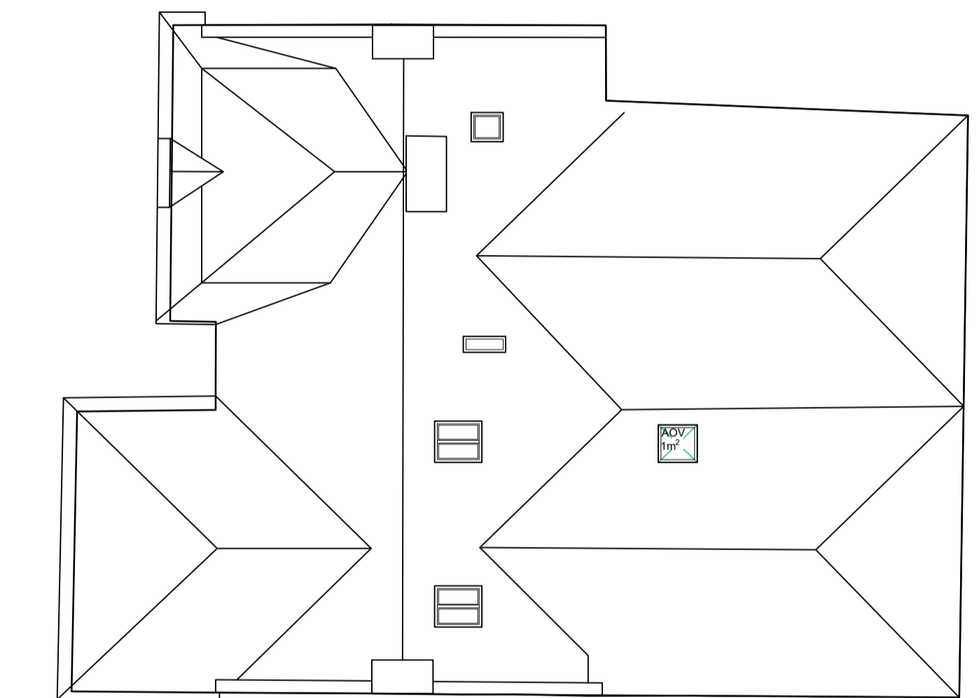
Roof Plan
