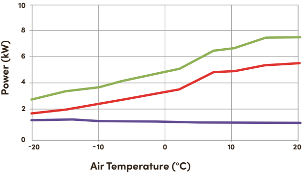
Castletown Performance at 35°C Outlet Temperature
