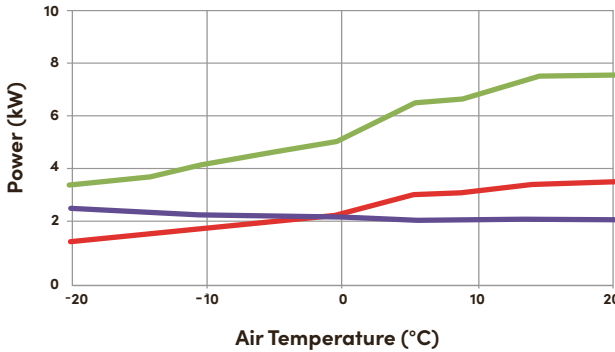
Castletown Performance at 55°C Outlet Temperature
