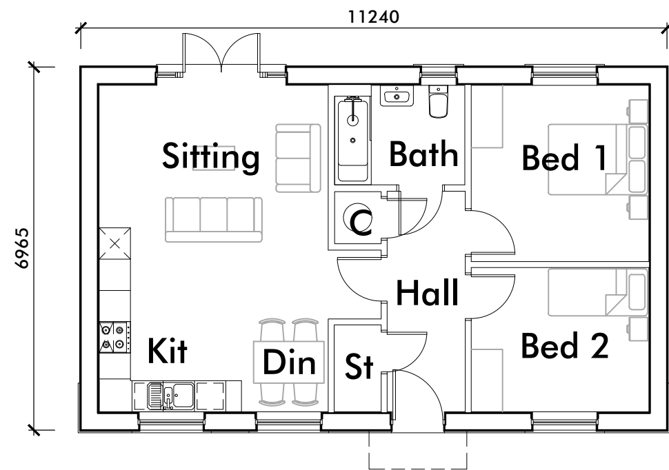
GF PLAN
