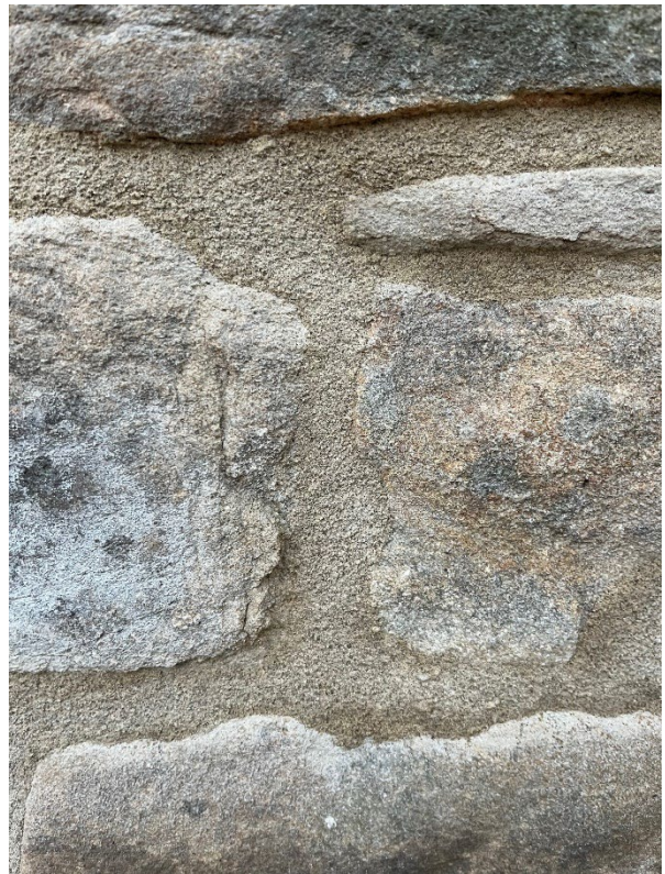
Sample images of re-pointing in lime – Between doorways on Northeast Elevation
