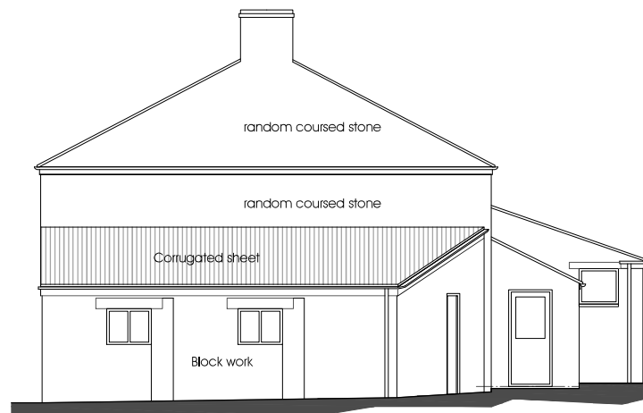
North East Elevation scale 1:100
