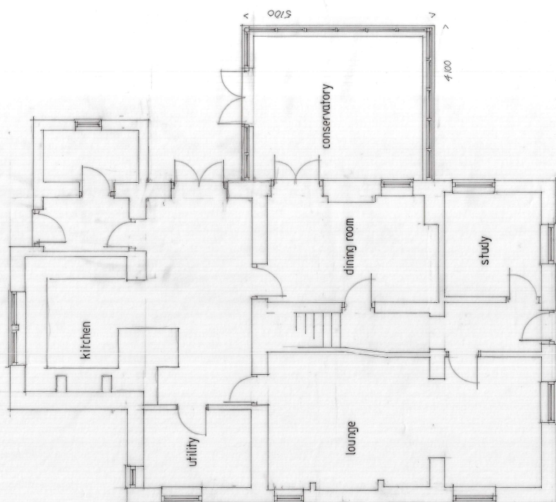
EXISTING PLAN
