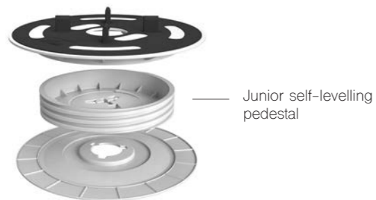
Junior Paving Pedestal J1 12mm - J3 30mm height
