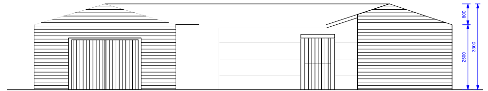
4 Elevation D - EXISTING 1:50 @ A1
