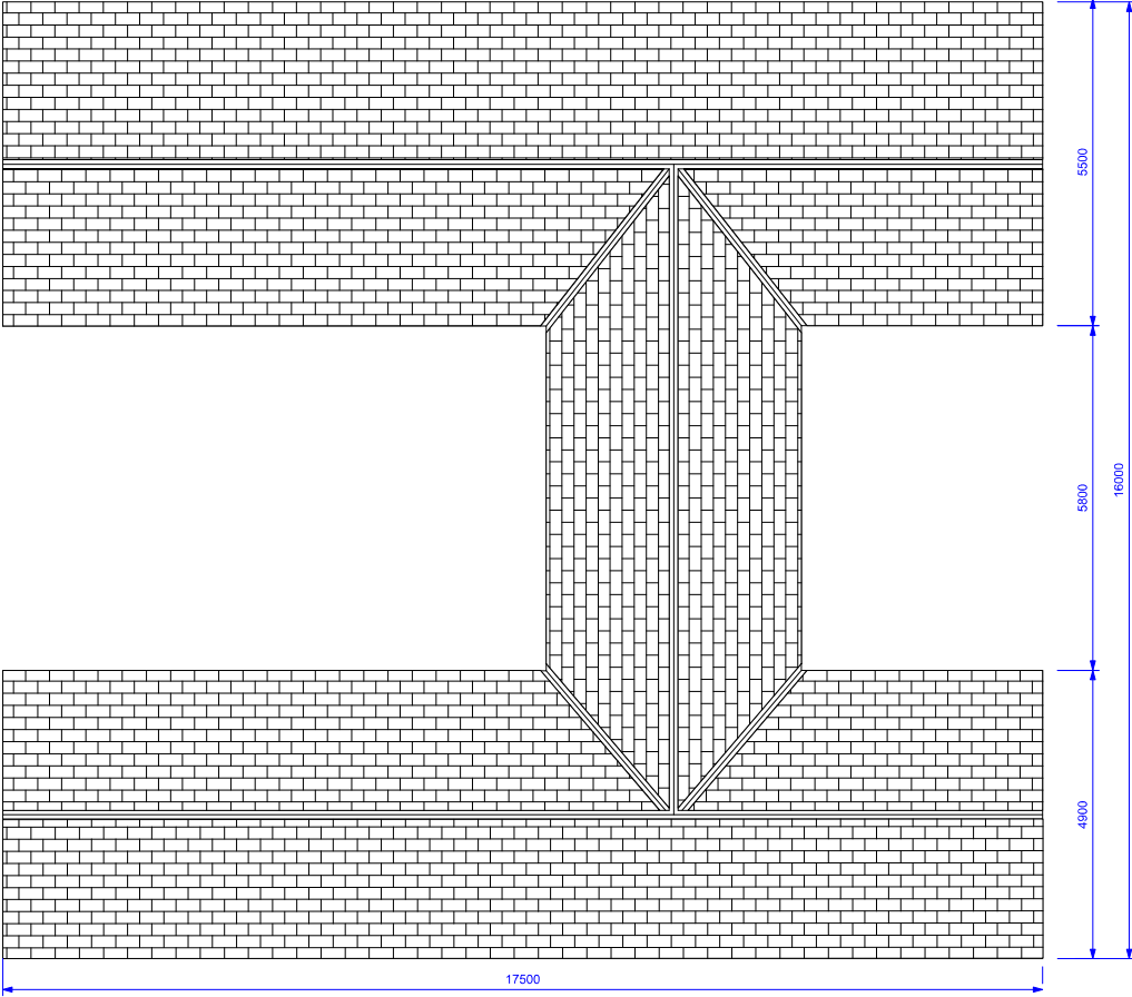
1 Roof Plan - Proposed 1:50 @ A1
