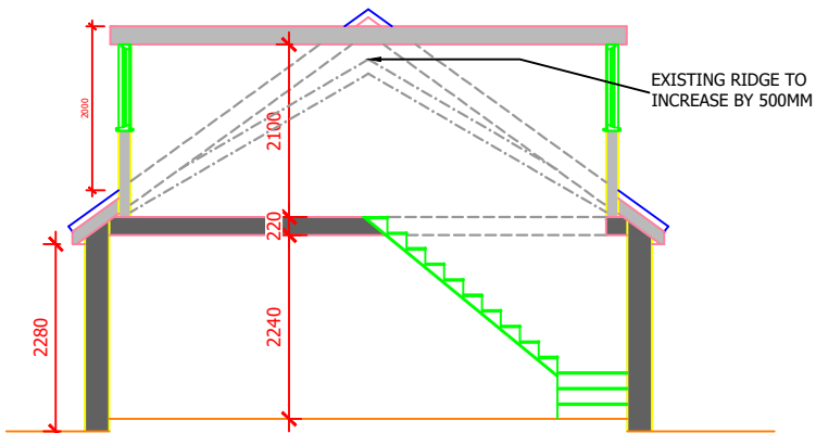
PROPOSED SECTION
