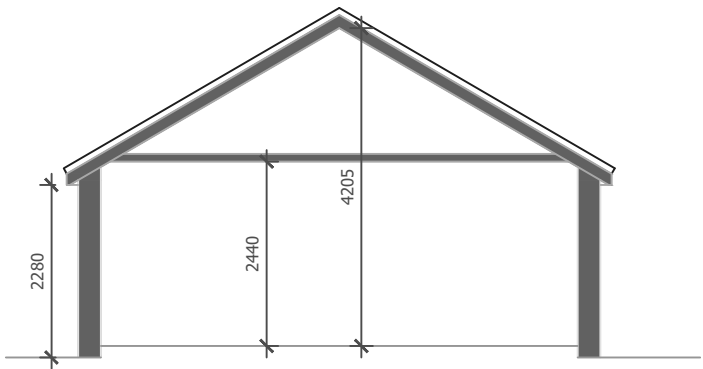
EXISTING SECTION
