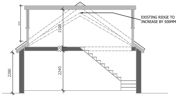
PROPOSED SECTION
