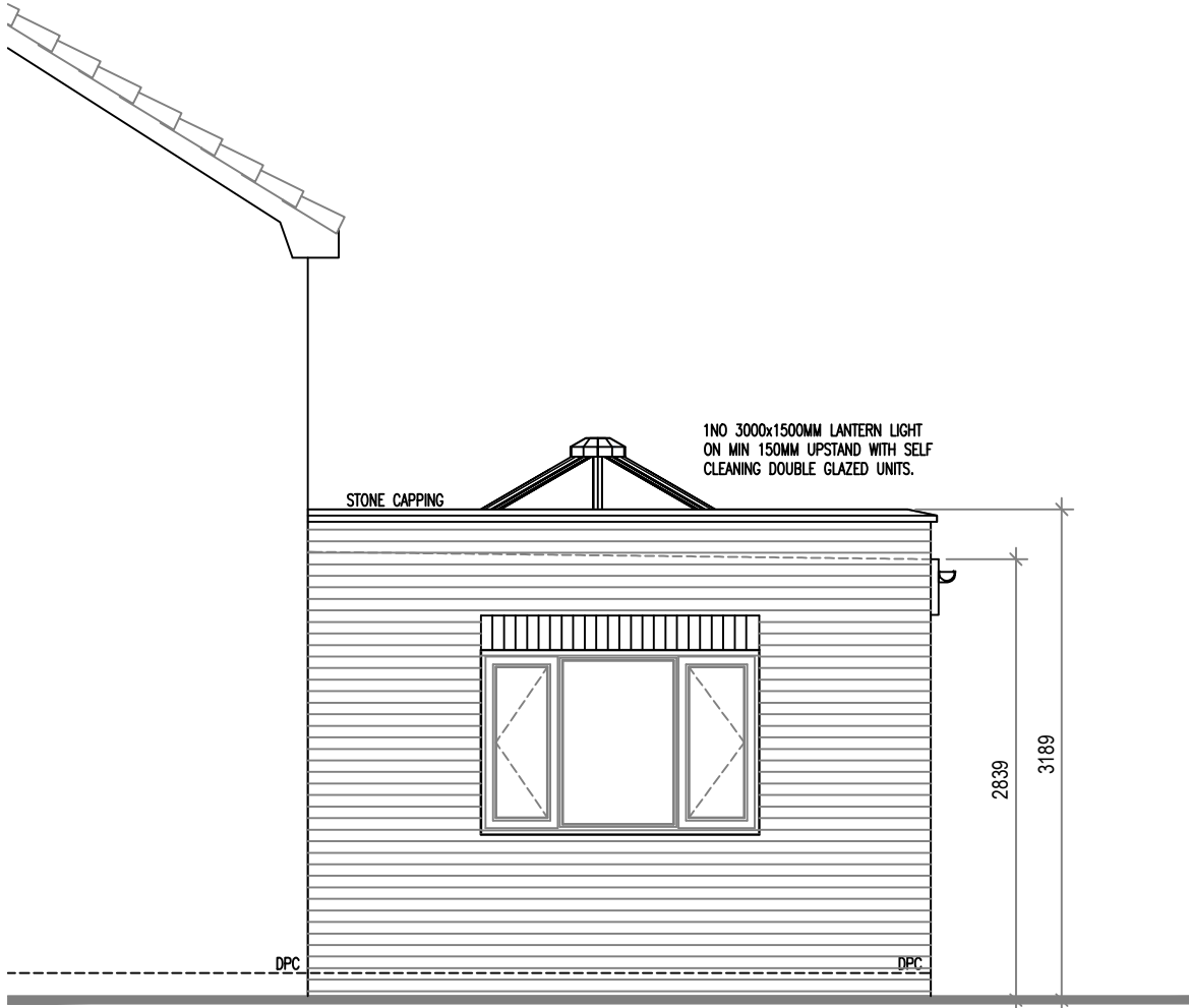
Side Elevation Partial
