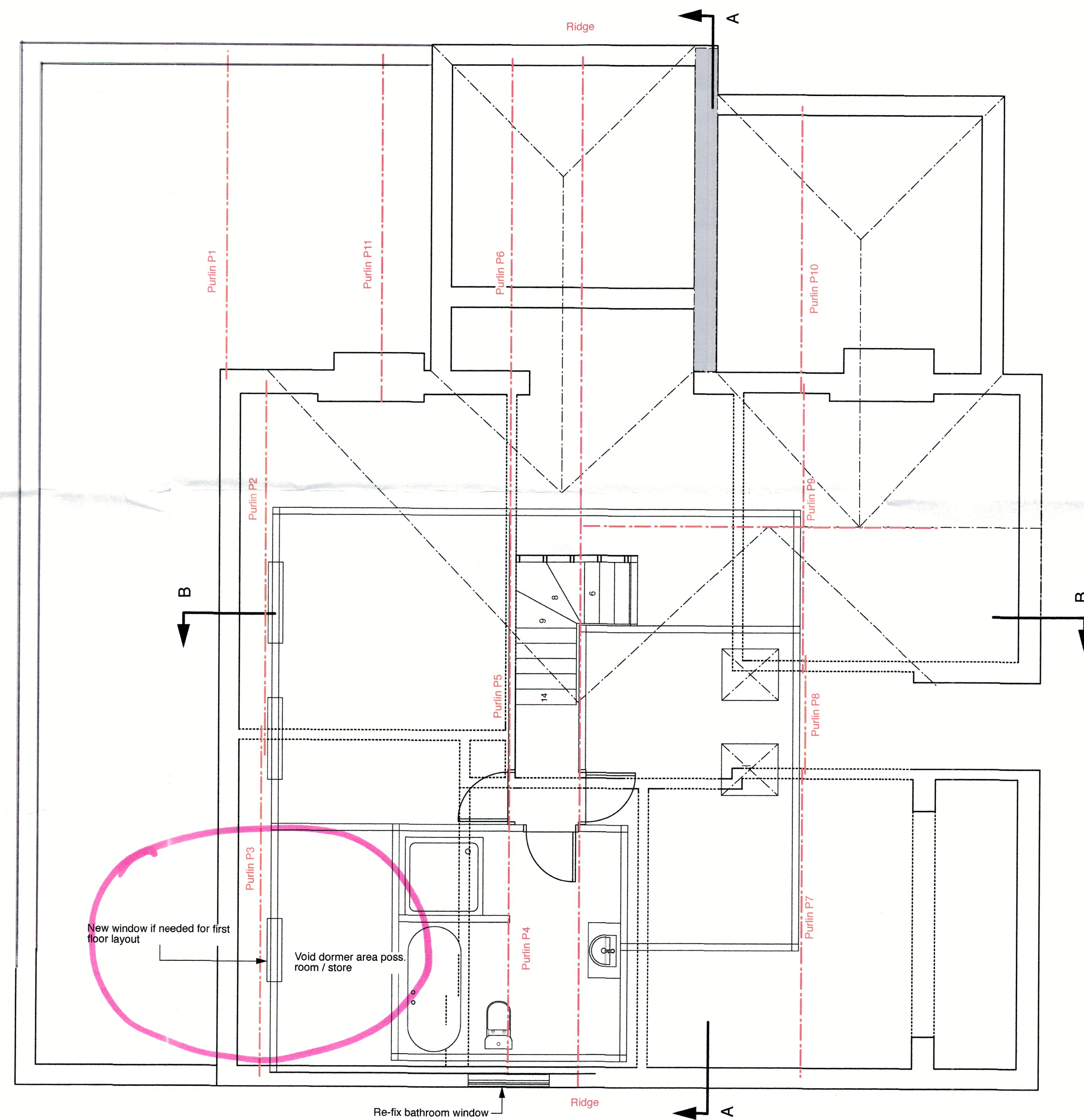
FIRST FLOOR PLAN PROPOSED (Amended 06/07/2025)
