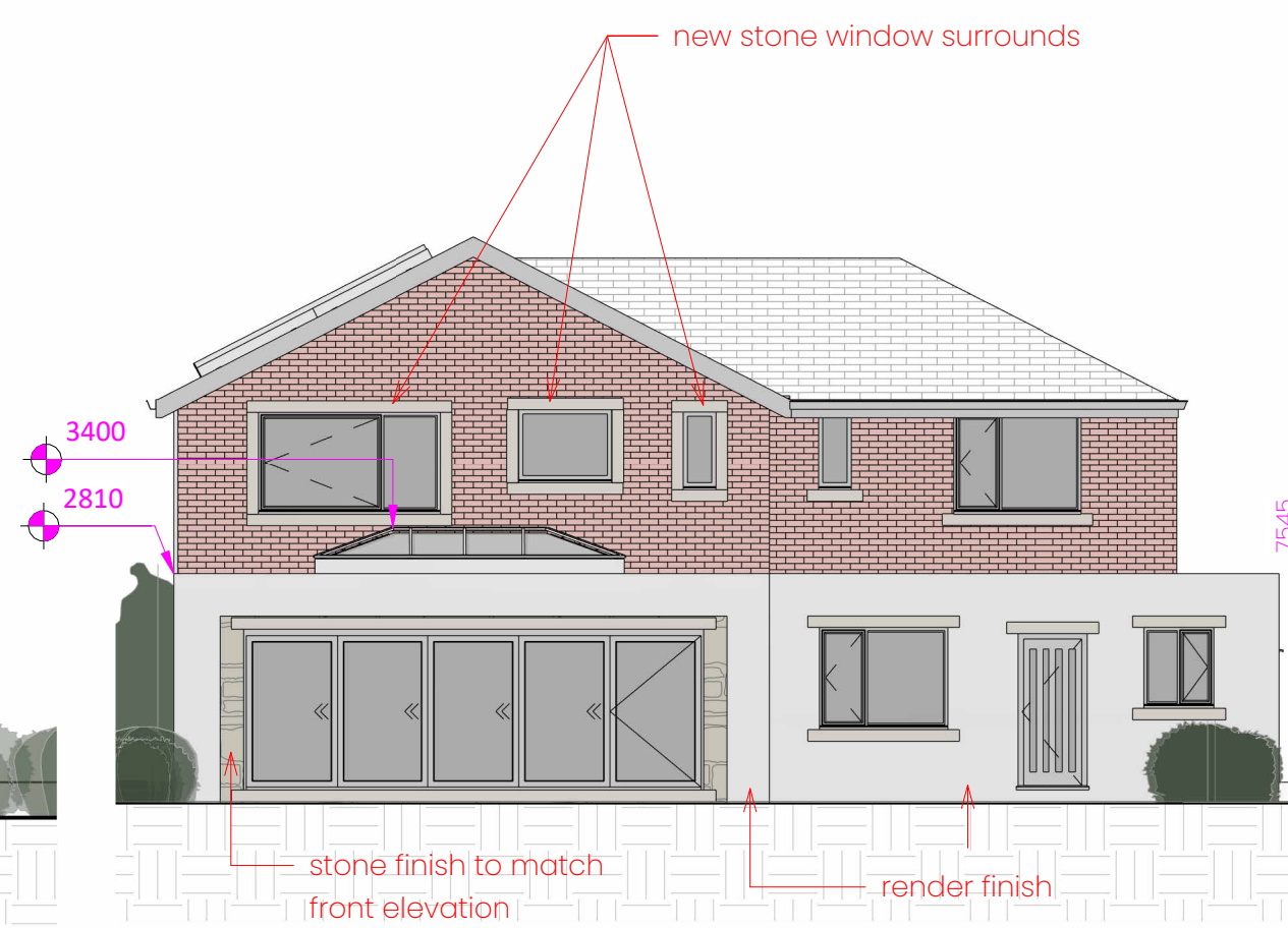
4 Proposed North East 1:100
