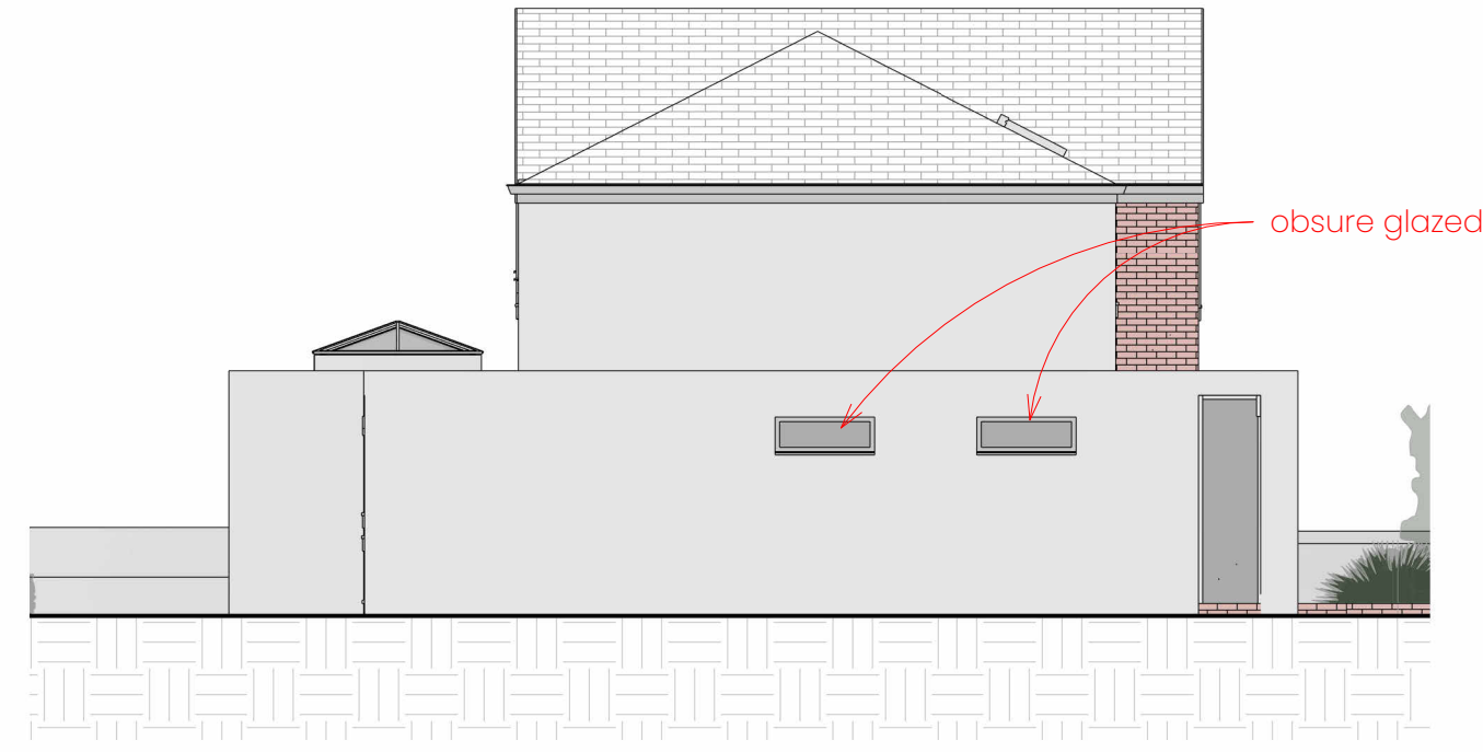
6 Proposed North West 1:100
