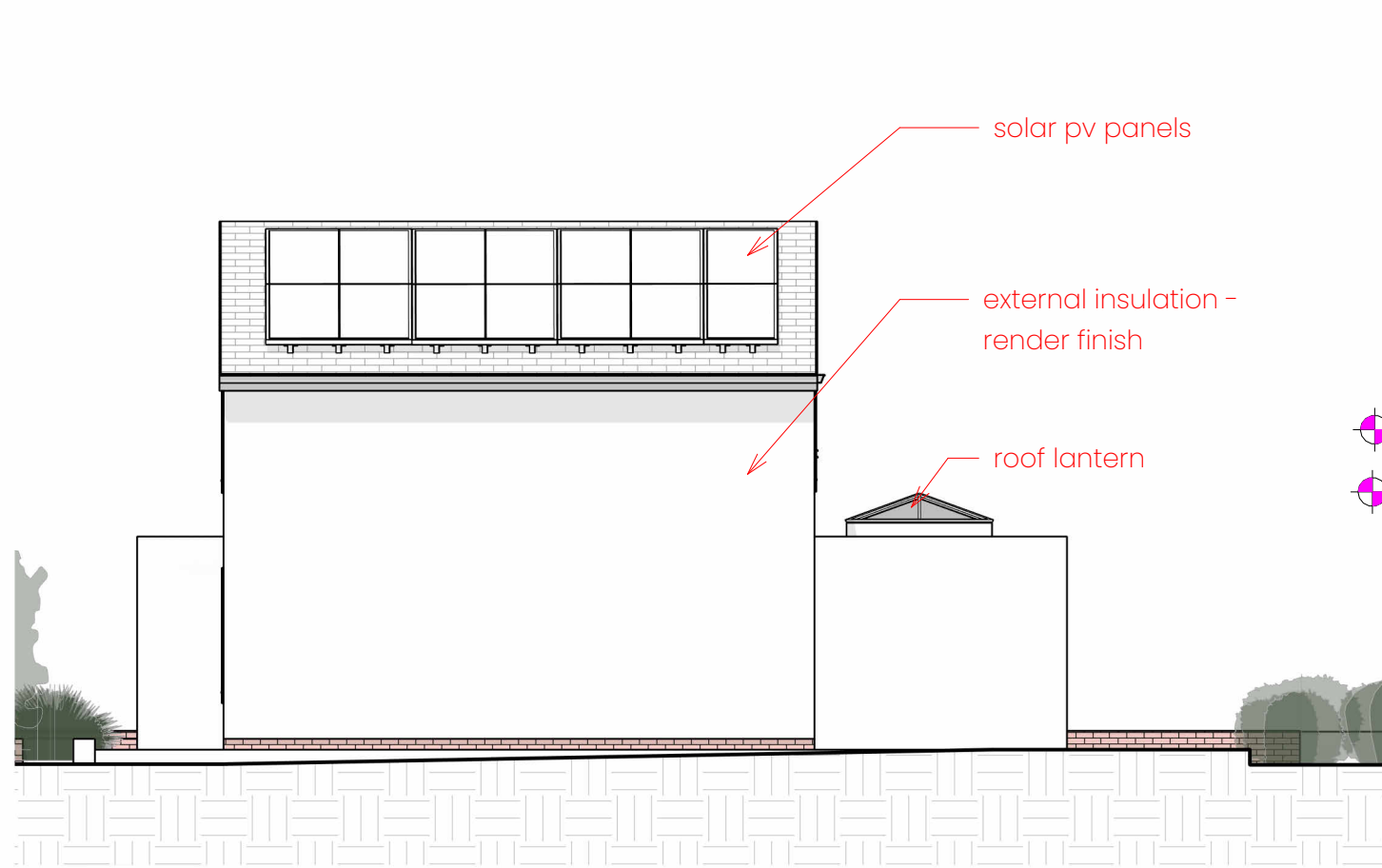
3 Proposed South East 1:100
