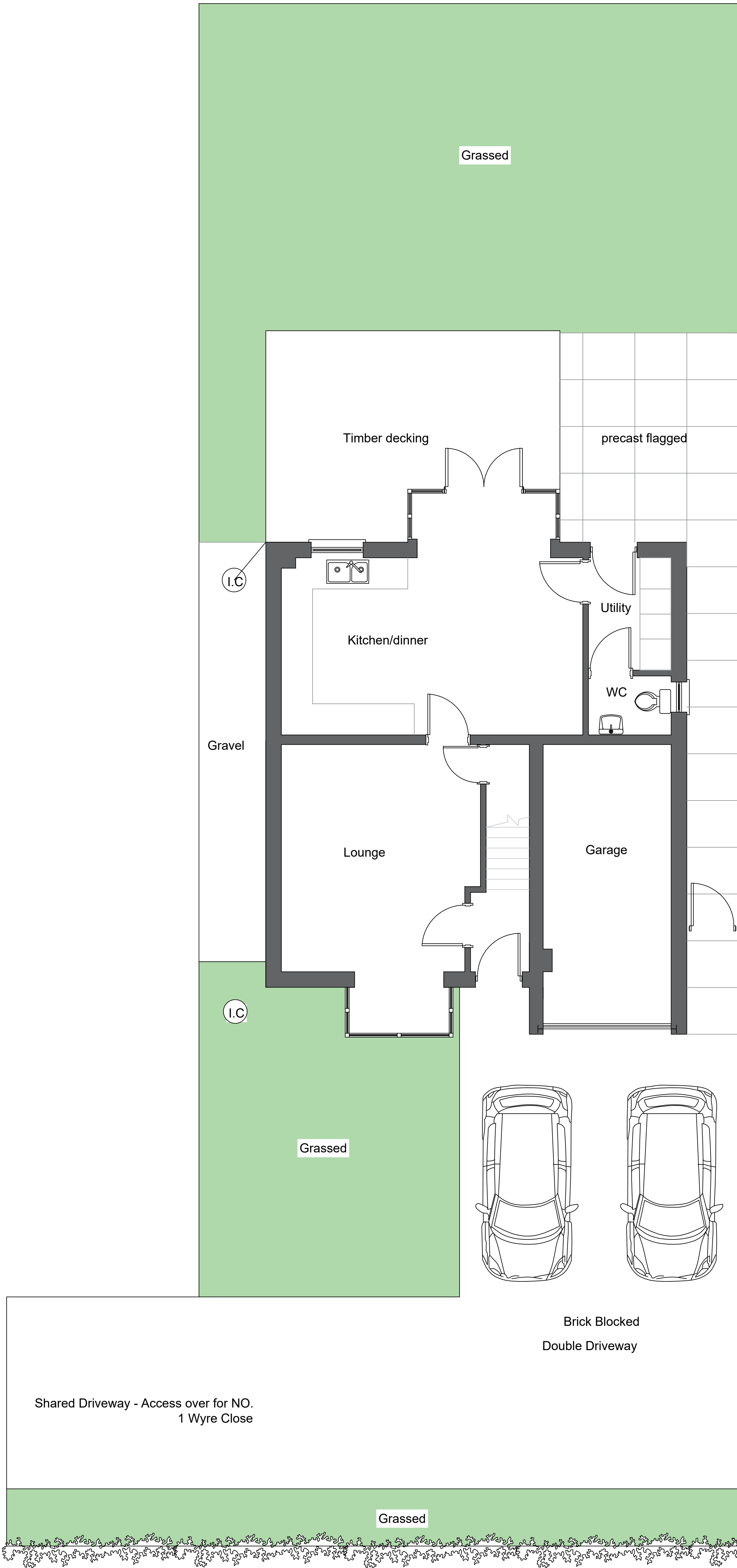
EXISTING GROUND FLOOR LAYOUT - SCALE 1 / 50 @ A0
