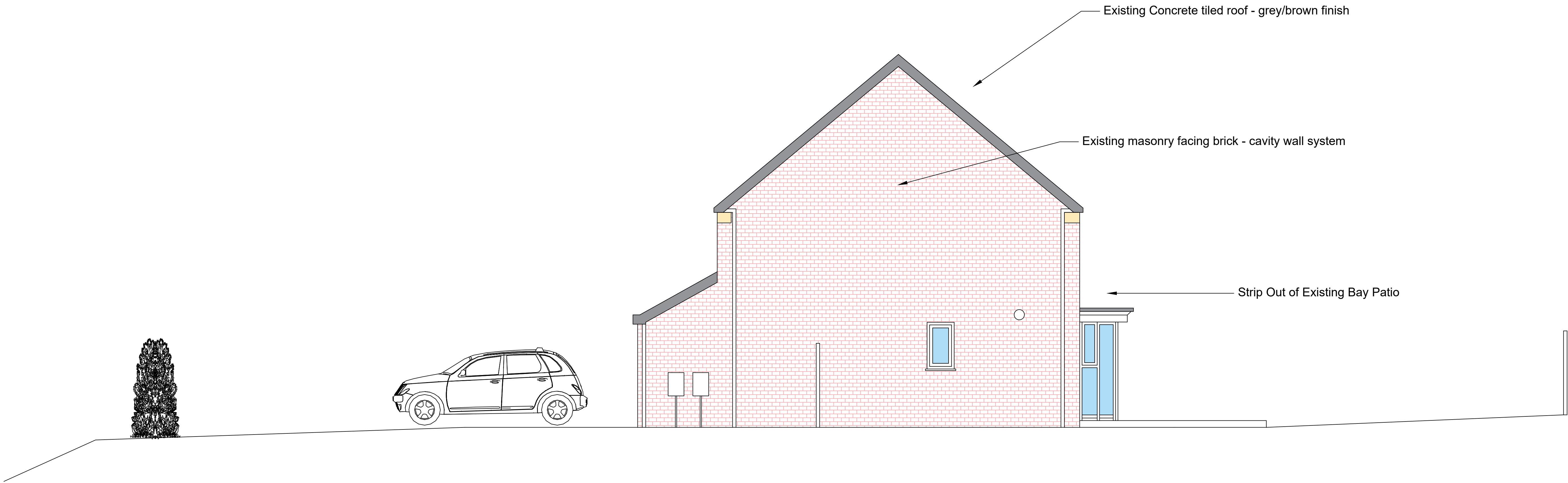
EXISTING WEST FACING ELEVATION - SCALE 1 / 50 @ A0
