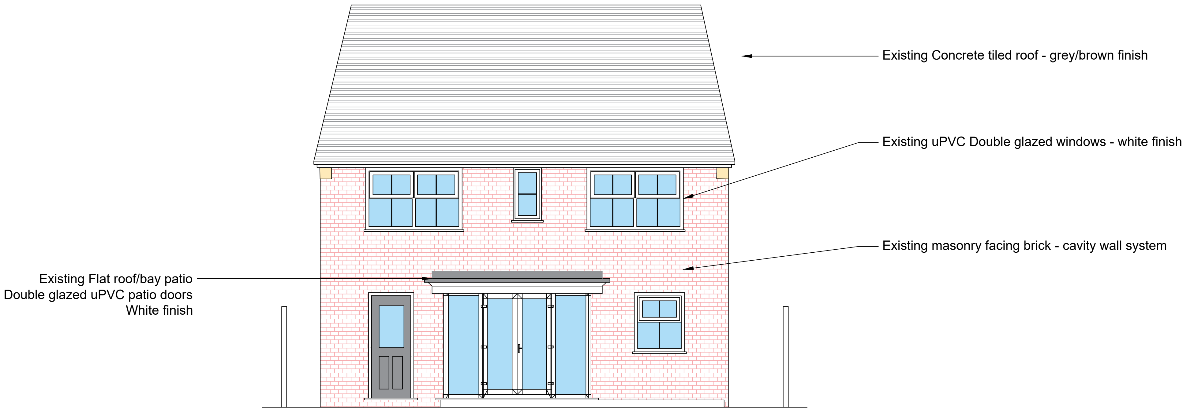
EXISTING SOUTH FACING ELEVATION - SCALE 1 / 50 @ A0
