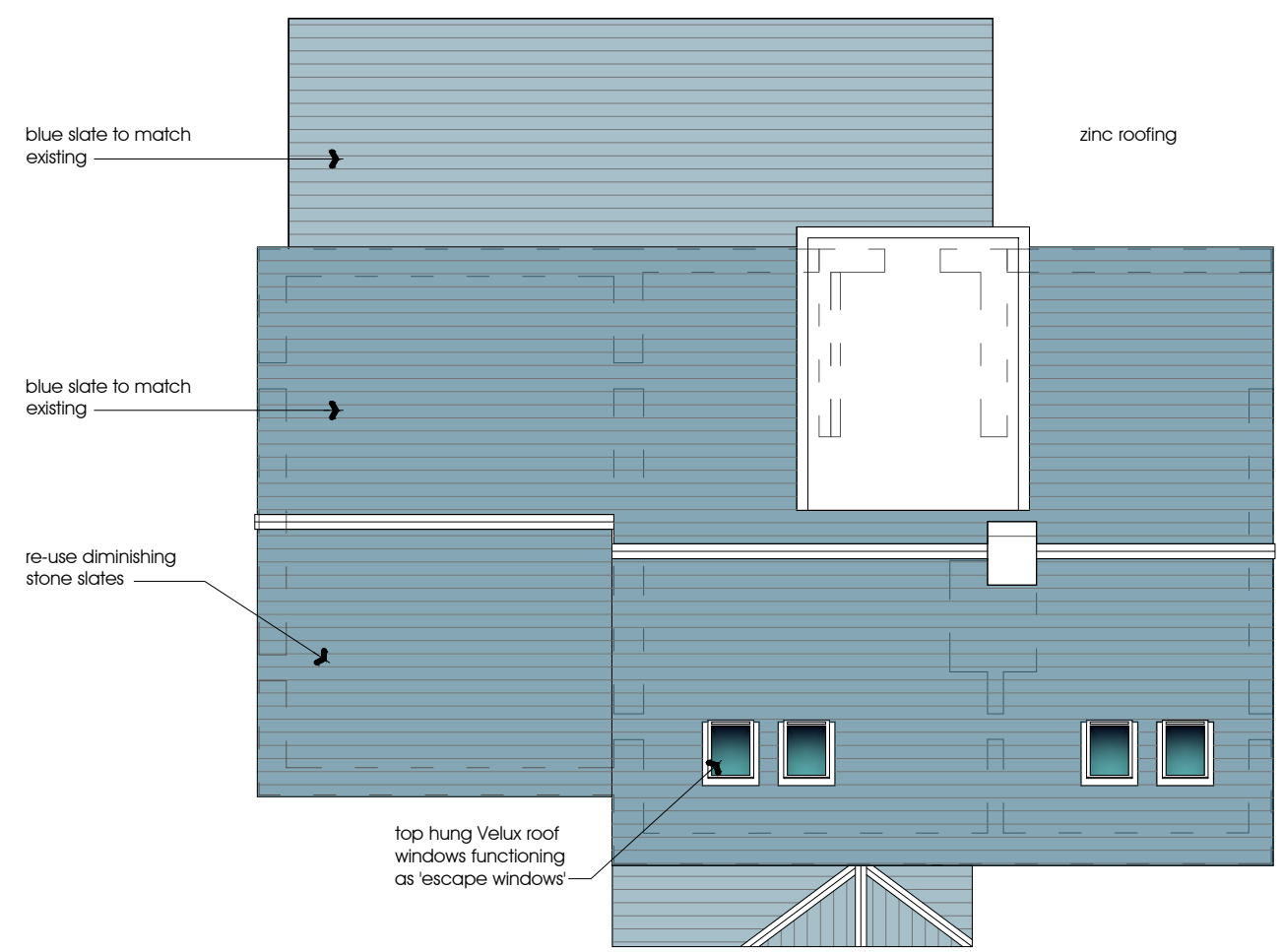
Roof Plan
