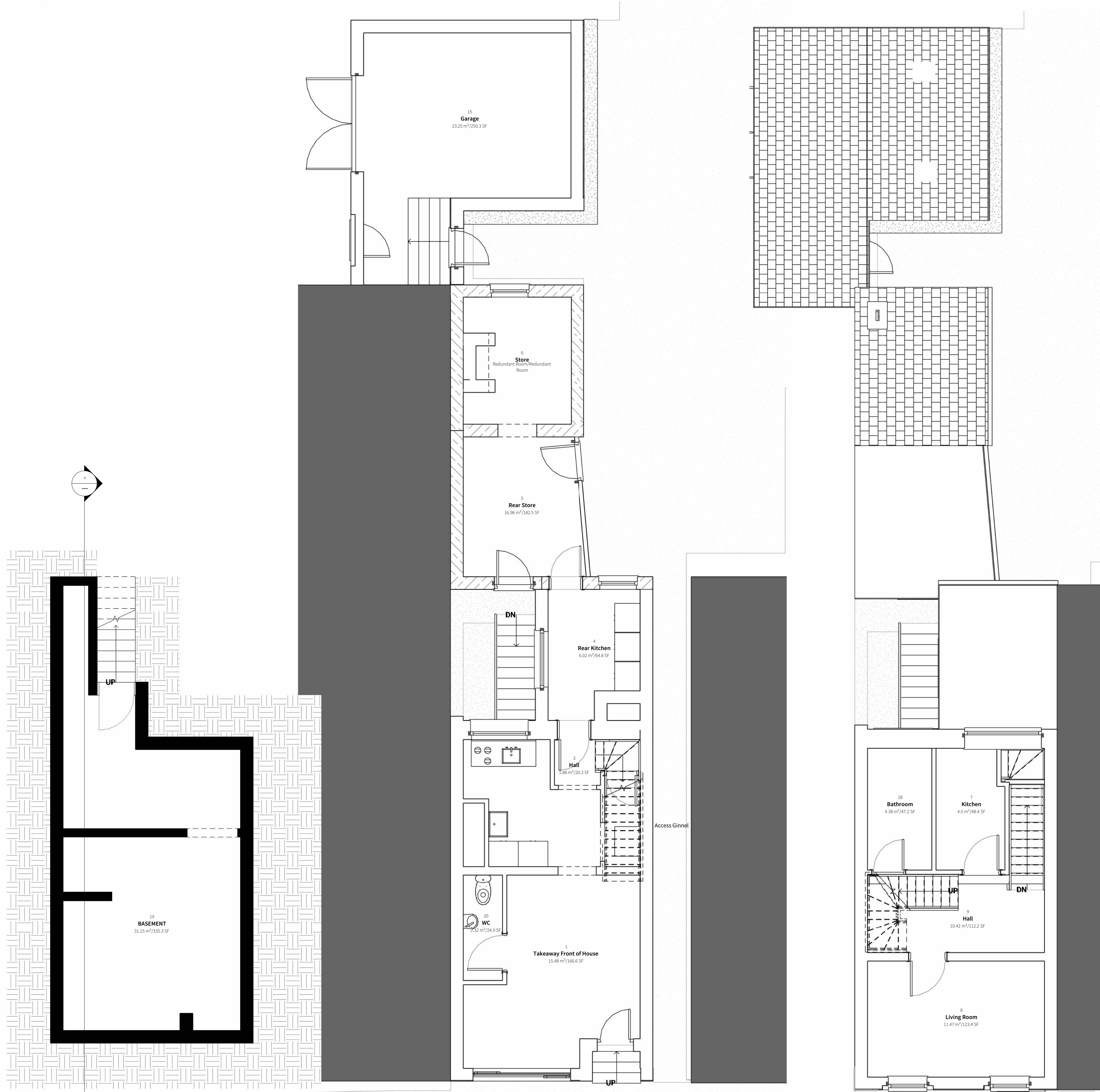
2 Existing Basement Floor Plan 1:50
