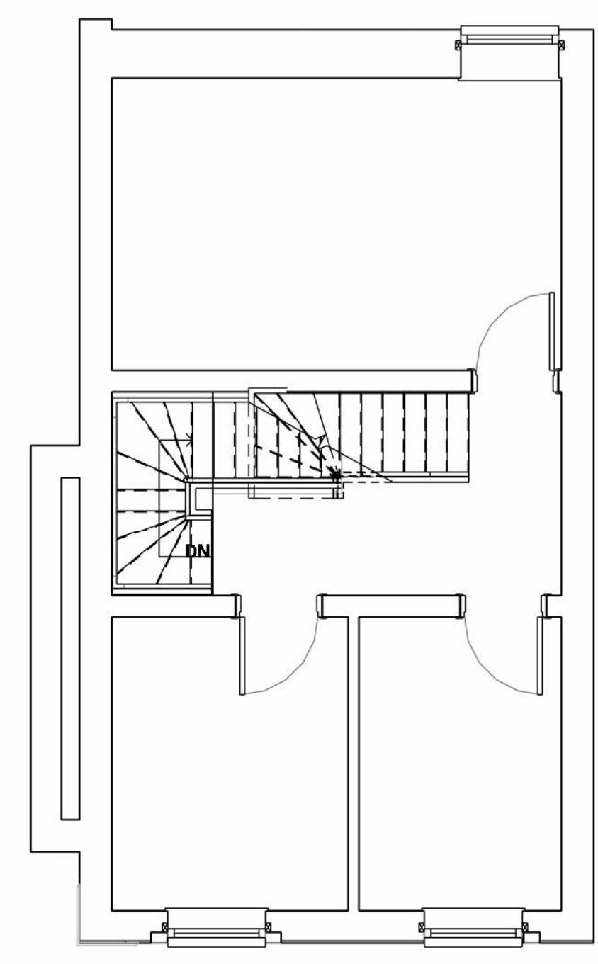
4 02-Second 1:50
