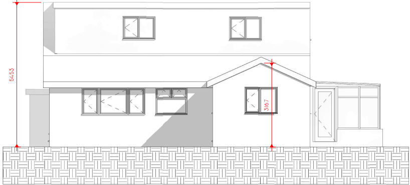
EXISTING SOUTH
