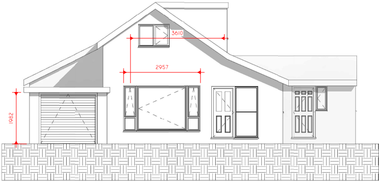
EXISTING WEST
