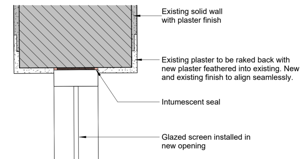
2 | Infill Glazed Screen Jamb Detail
