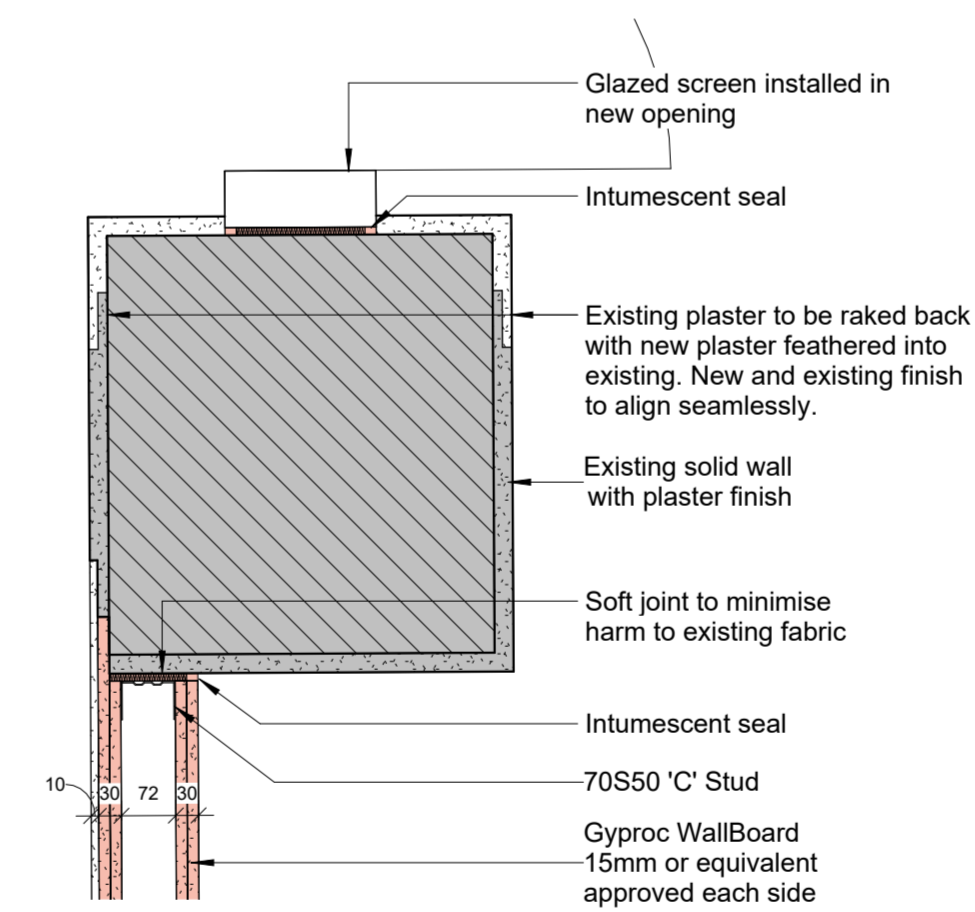
4 | Wall Infill Plan Detail
