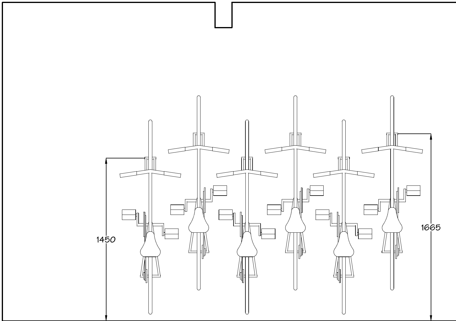
Elevation of vertical offset cycle storage
