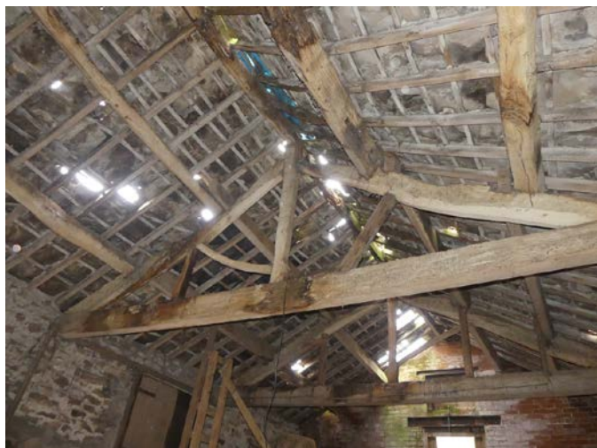
Plate 89 (left): North-east truss, Room F2 of the barn, viewed from the north
