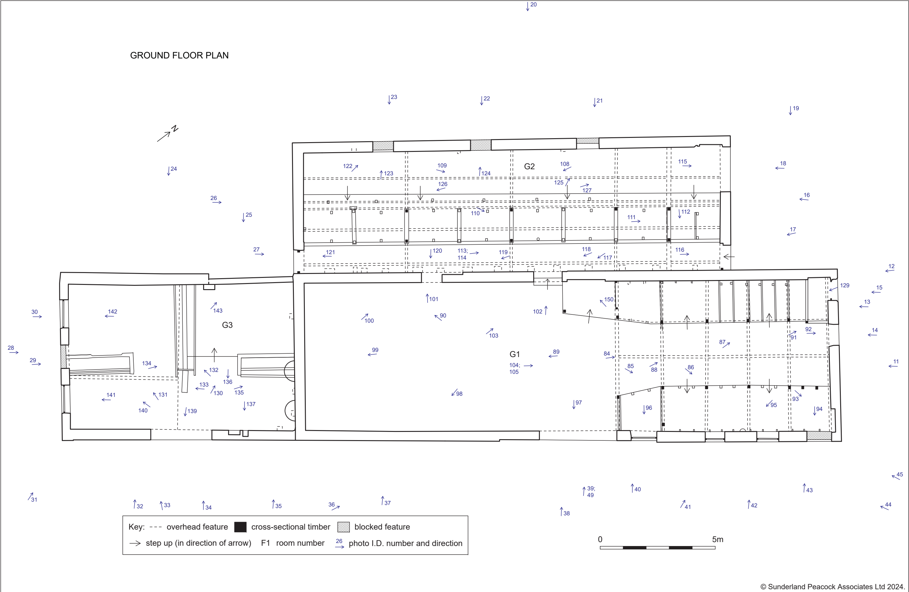
Figure 11: Ground floor plan of the barn, showing the location and direction of photographs taken
