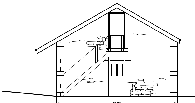
South Elevation
