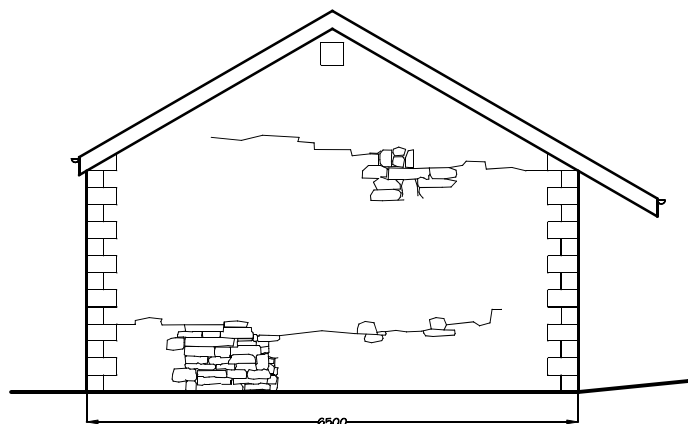
North Elevation
