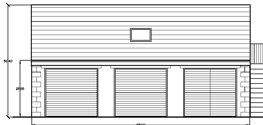
West Elevation
