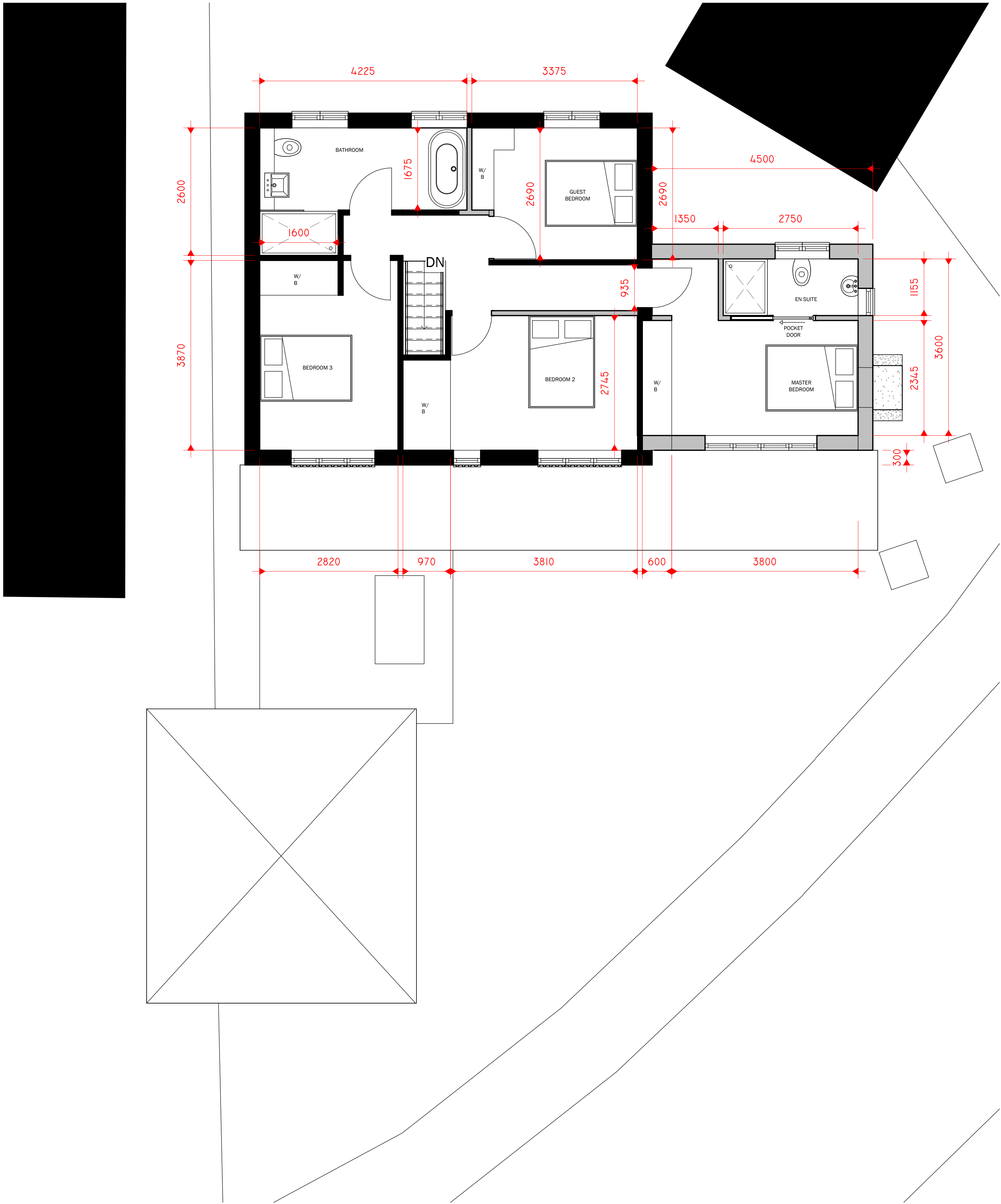
1 PROPOSED FIRST FLOOR 1 : 50
