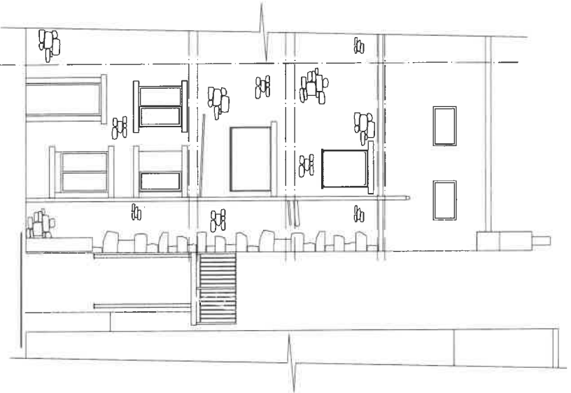
Rear Elevation (North) 1:50 Scale
