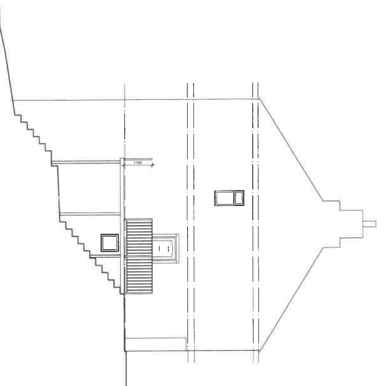
Side Elevation (West) 1:50 Scale
