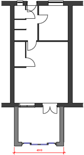
4 0 PROPOSED GROUND FLOOR 1 : 50
