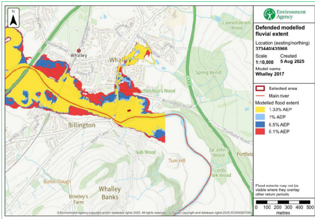
Figure 6 - Environment Agency Defended Modelled Flood Outlines
