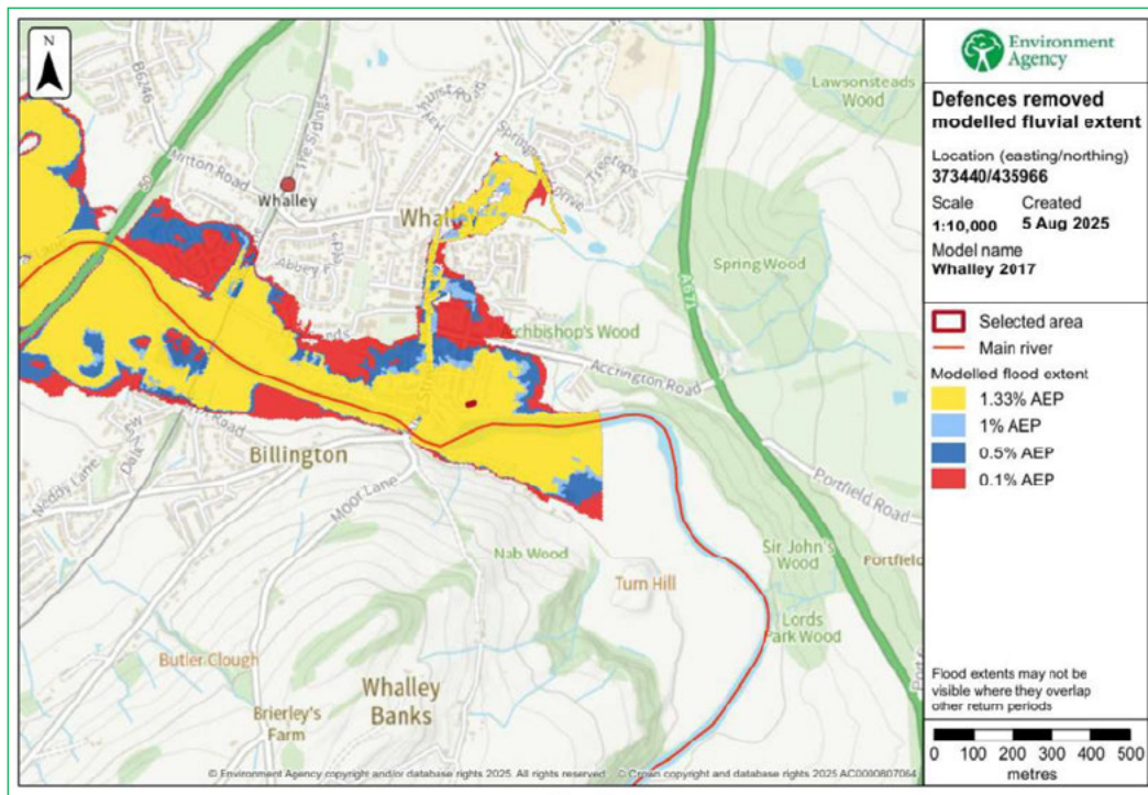
Figure 8 - Environment Agency Undefended Modelled Flood Outlines
