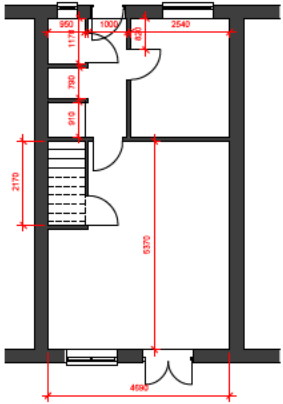
1 0 GROUND FLOOR 1 : 50
