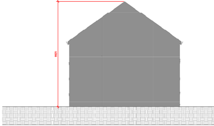
5 EXISTING EAST 1 : 50
