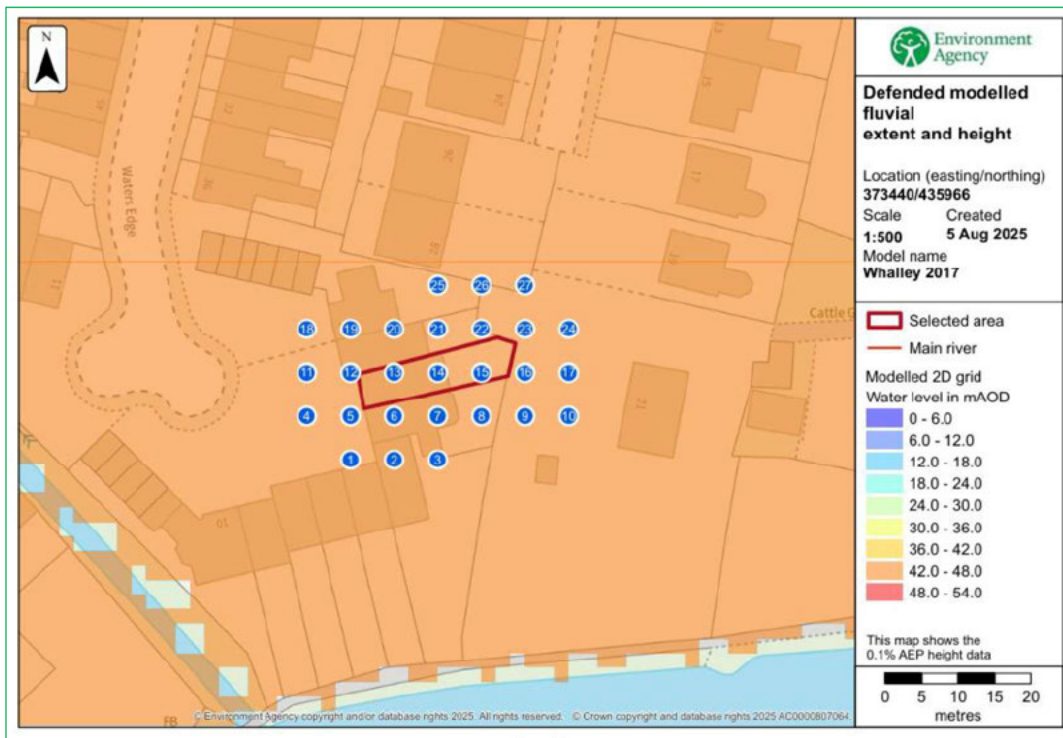
Figure 5 - Environment Agency Modelled Nodes Location Map
