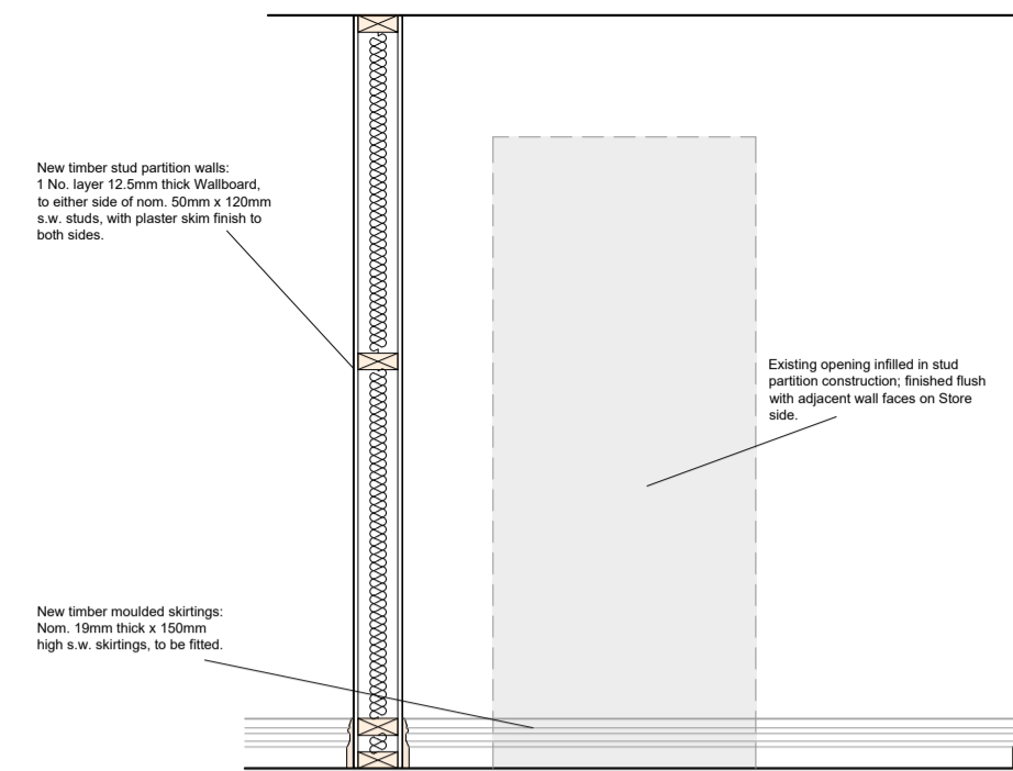
Store (Adjacent to Pantry). Scale 1:25
