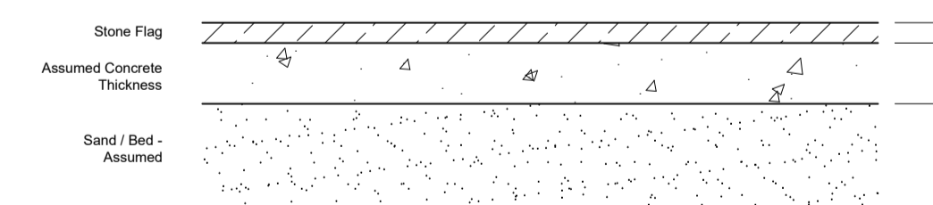
Existing Floor Build-Up. Scale 1:10
