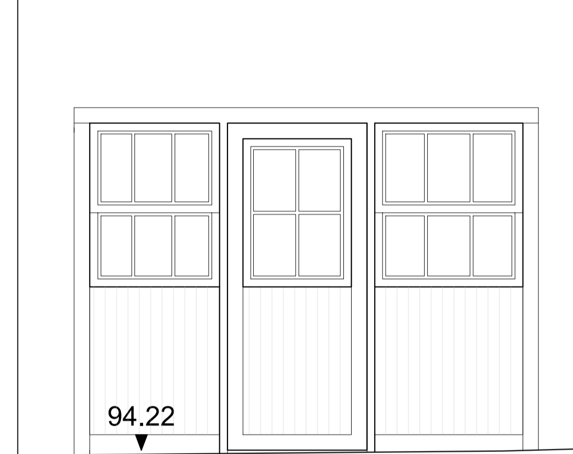
Outbuilding External Door Alterations Scale 1:25
