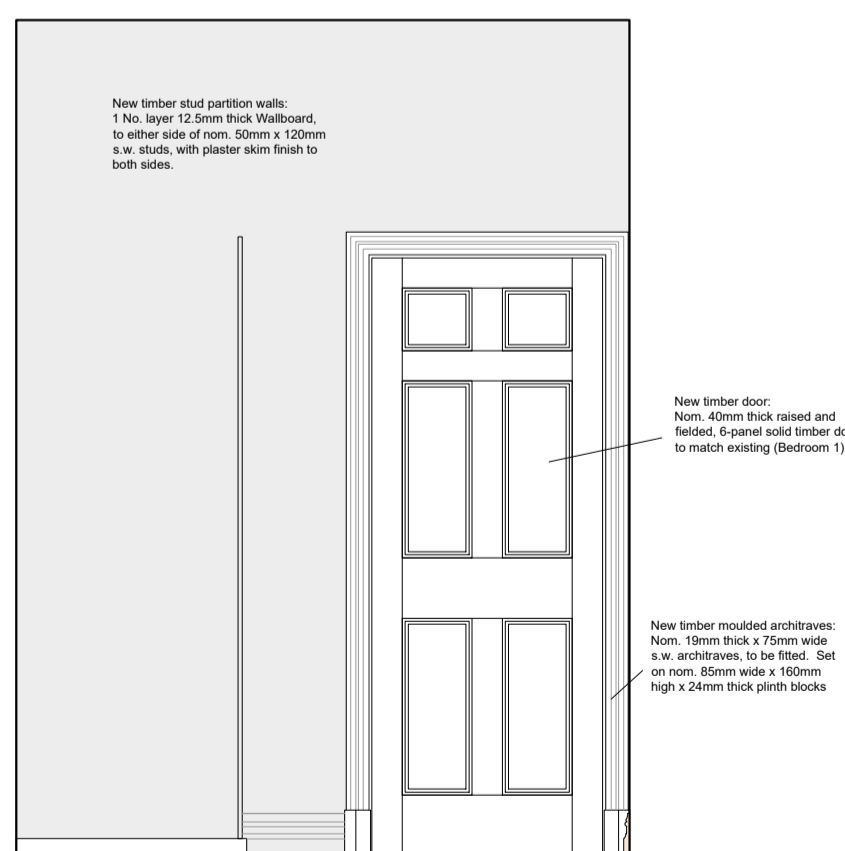
Bedroom 5 En Suite (Looking Towards Bedroom 5). Scale 1:25
