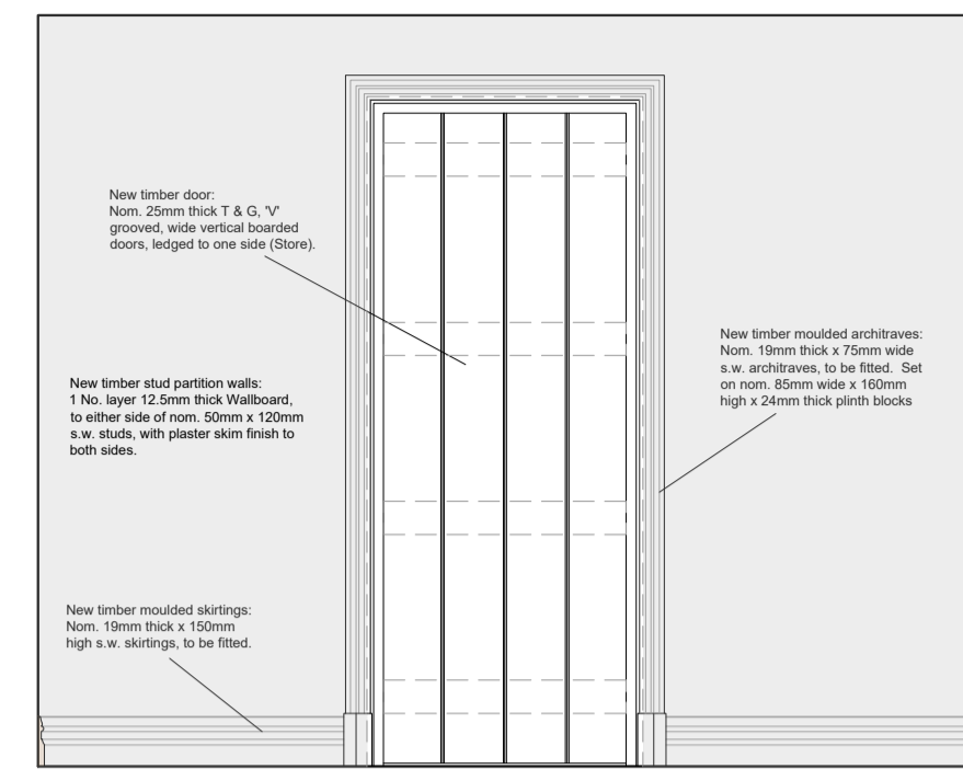
Pantry (Looking Towards Store). Scale 1:25
