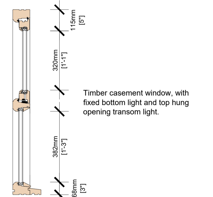
Proposed Section Through Casement Window Scale 1:10
