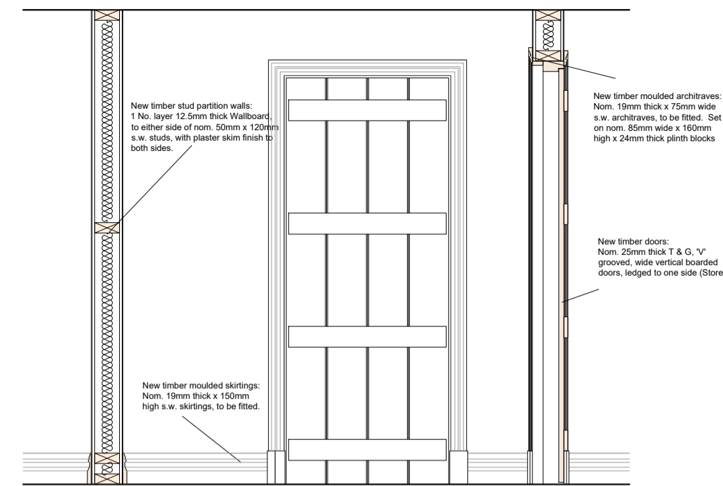
Section Through Pantry (Looking Towards Kitchen). Scale 1:25
