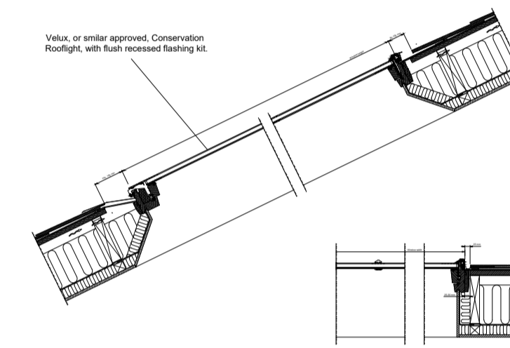
Outbuilding Typical Conservation Rooflight. Scale 1:25
