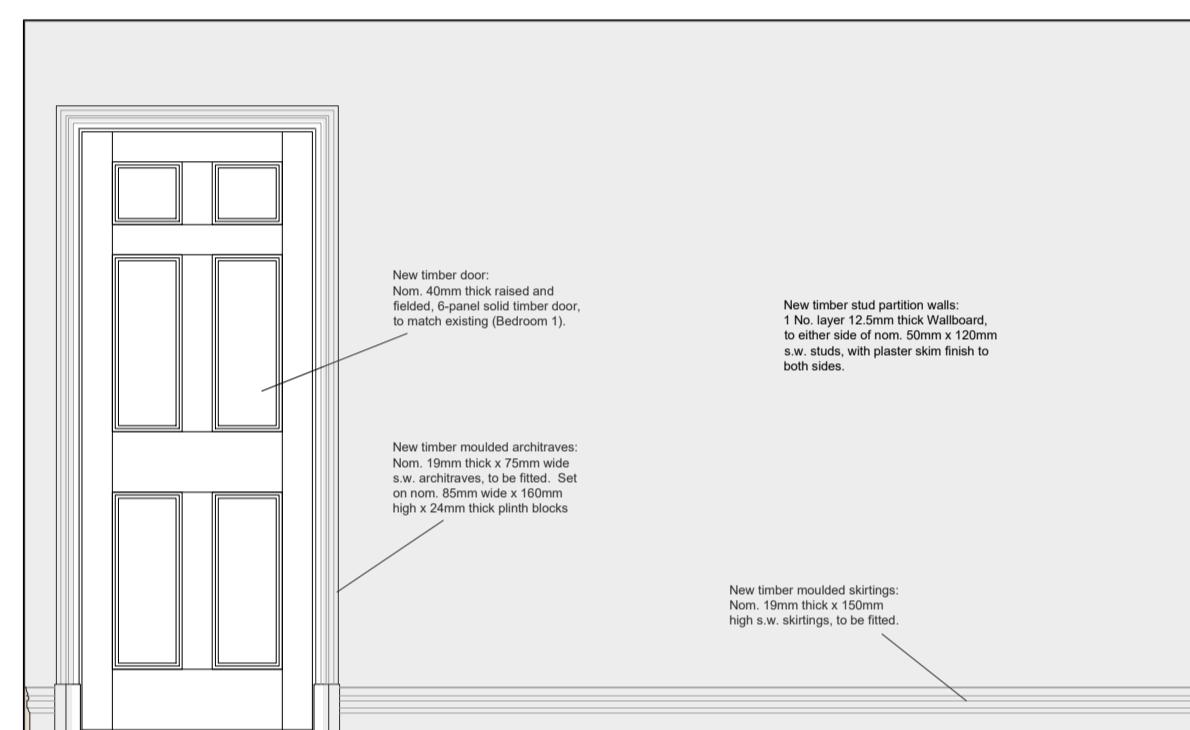
Bedroom 1 (Looking Towards FF Landing). Scale 1:25
