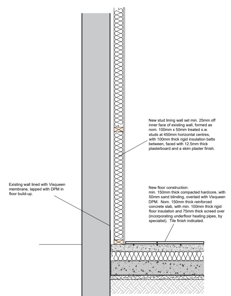
Outbuilding Floor and Lining Wall. Scale 1:25
