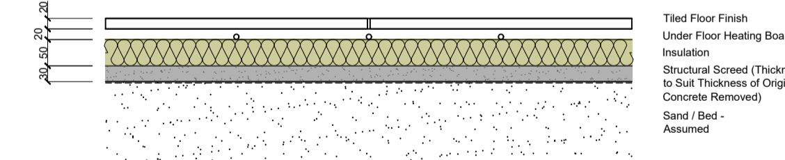
Proposed Floor Build-Up. Scale 1:10
