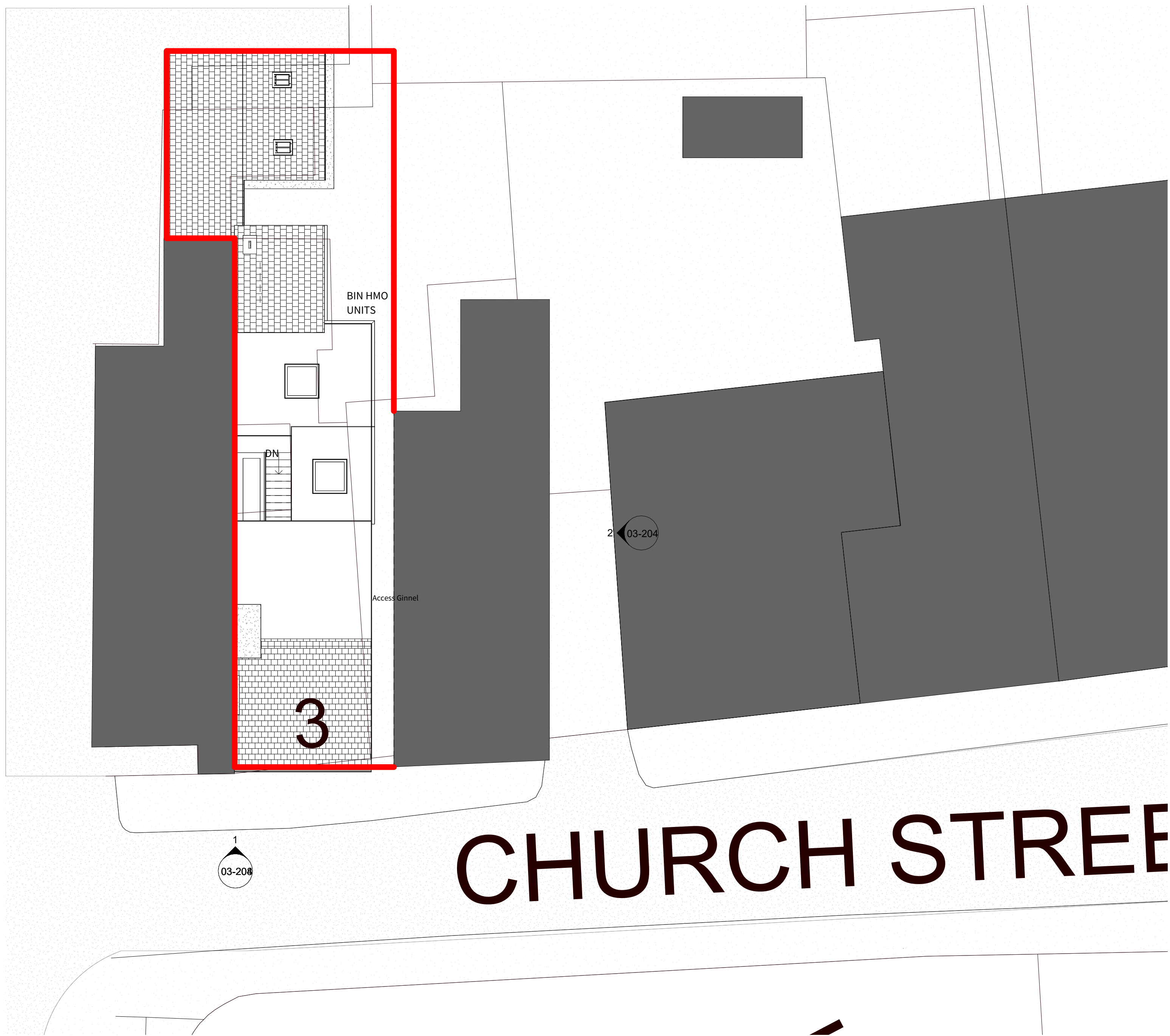
1 Proposed Site Plan 1:100
