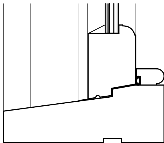
Vertical Section 1:2
