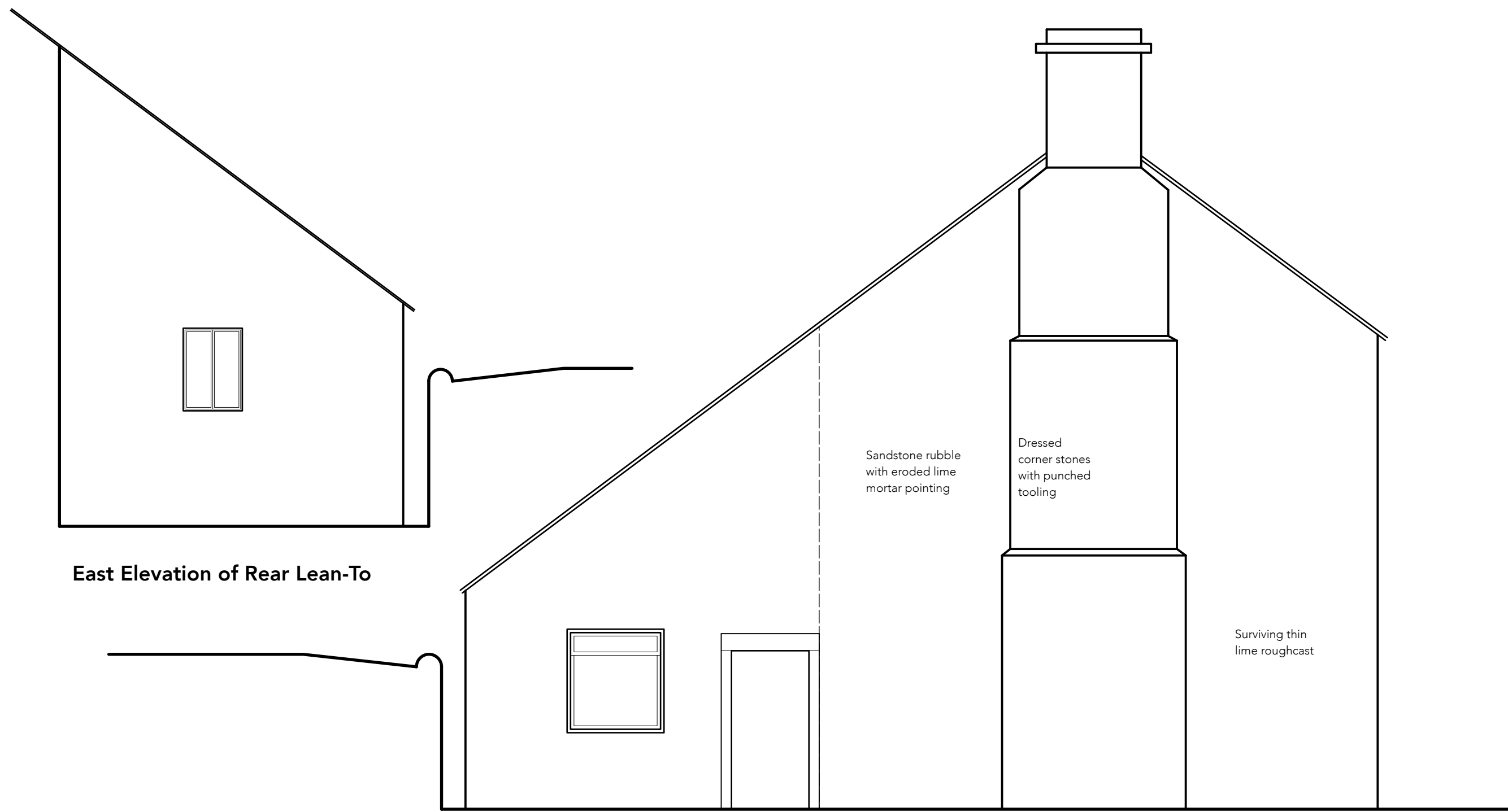
West Gable Elevation
