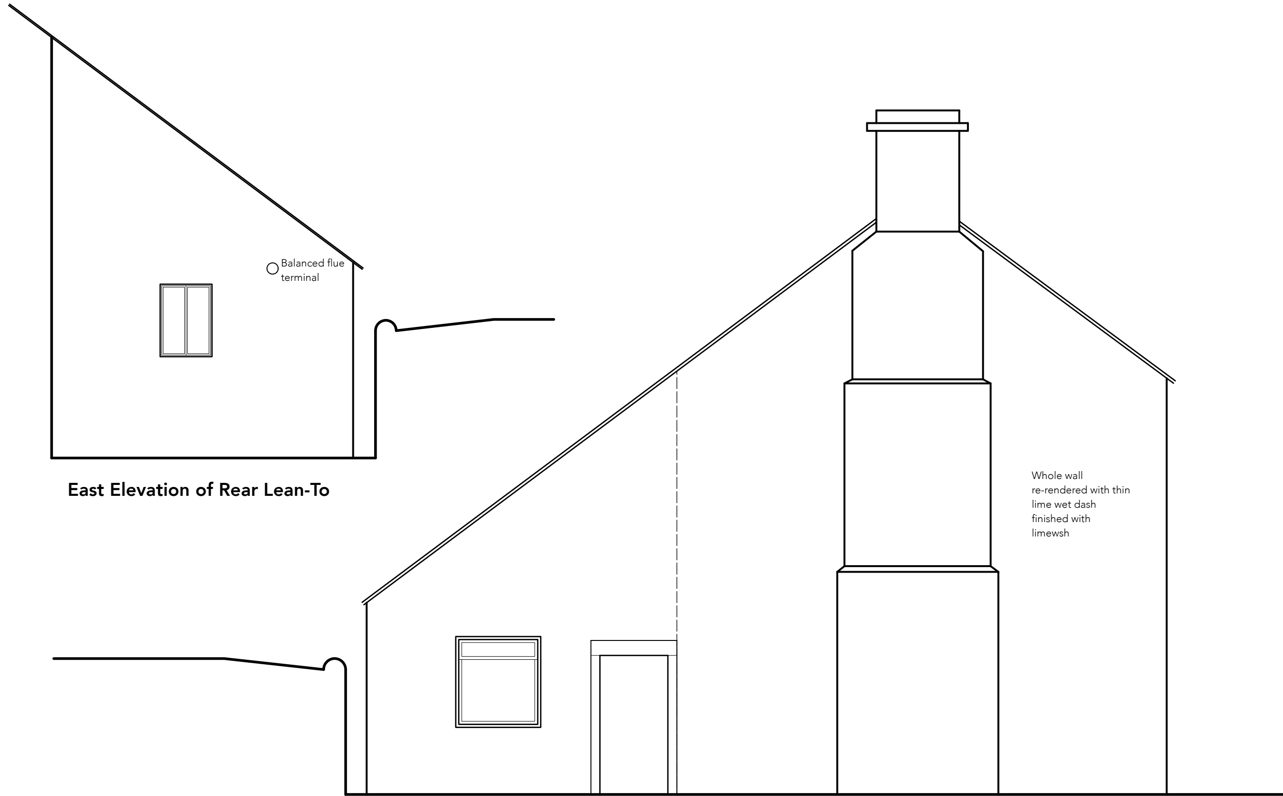
West Gable Elevation
