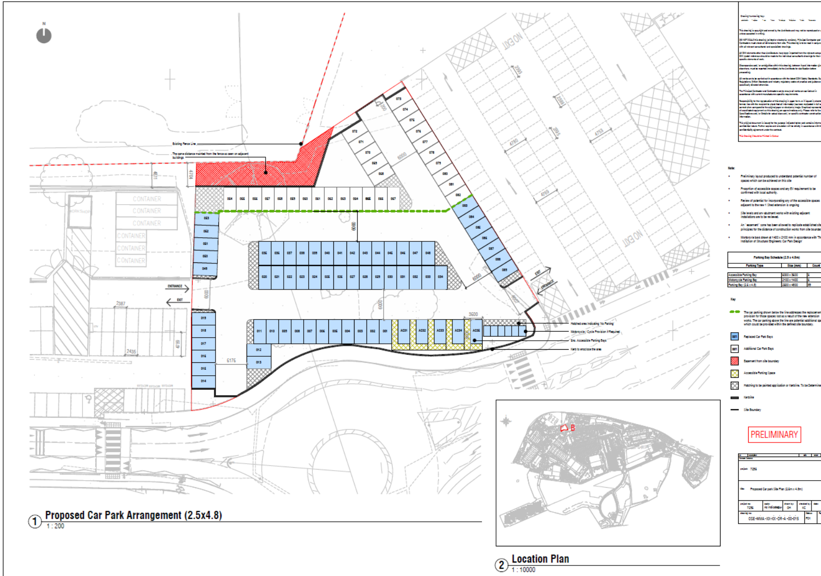
Figure 2: Site Proposals (drawing no: OSE-WMA-XX-XX-DR-A-00-014)
