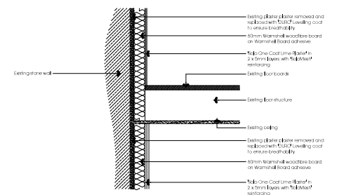
First Floor to Wall Junction detail
