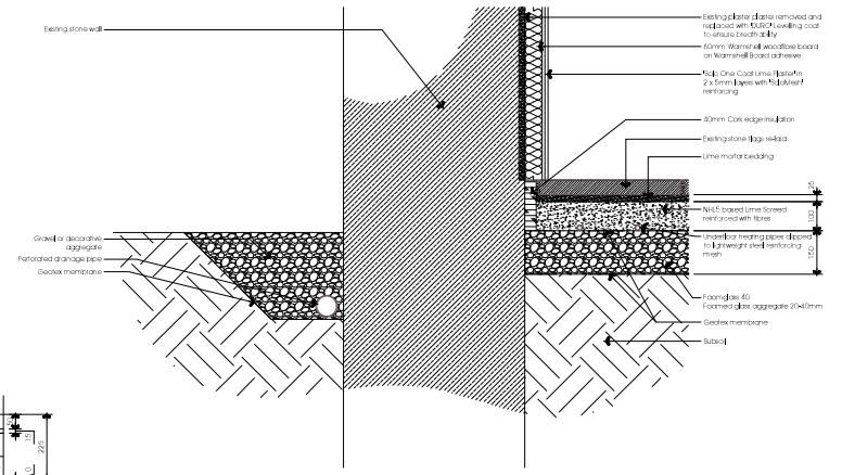
Ground Floor to Wall Junction detail
