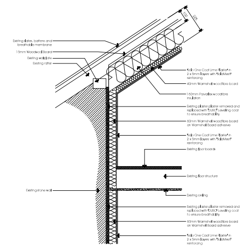
Second Floor to Wall and Roof Junction detail
