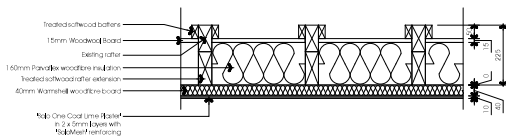
Roof - Rafter Level Insulation Detail
