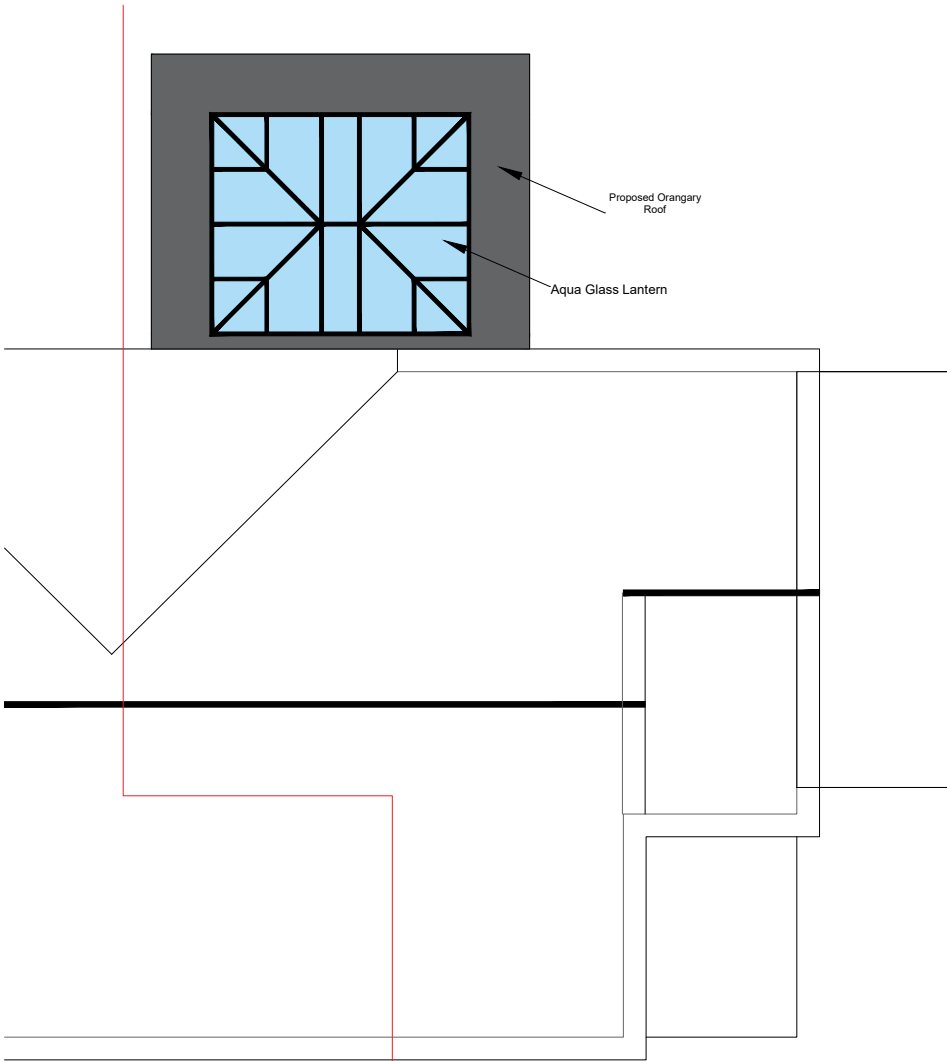
PROPOSED ROOF FLOOR PLAN
