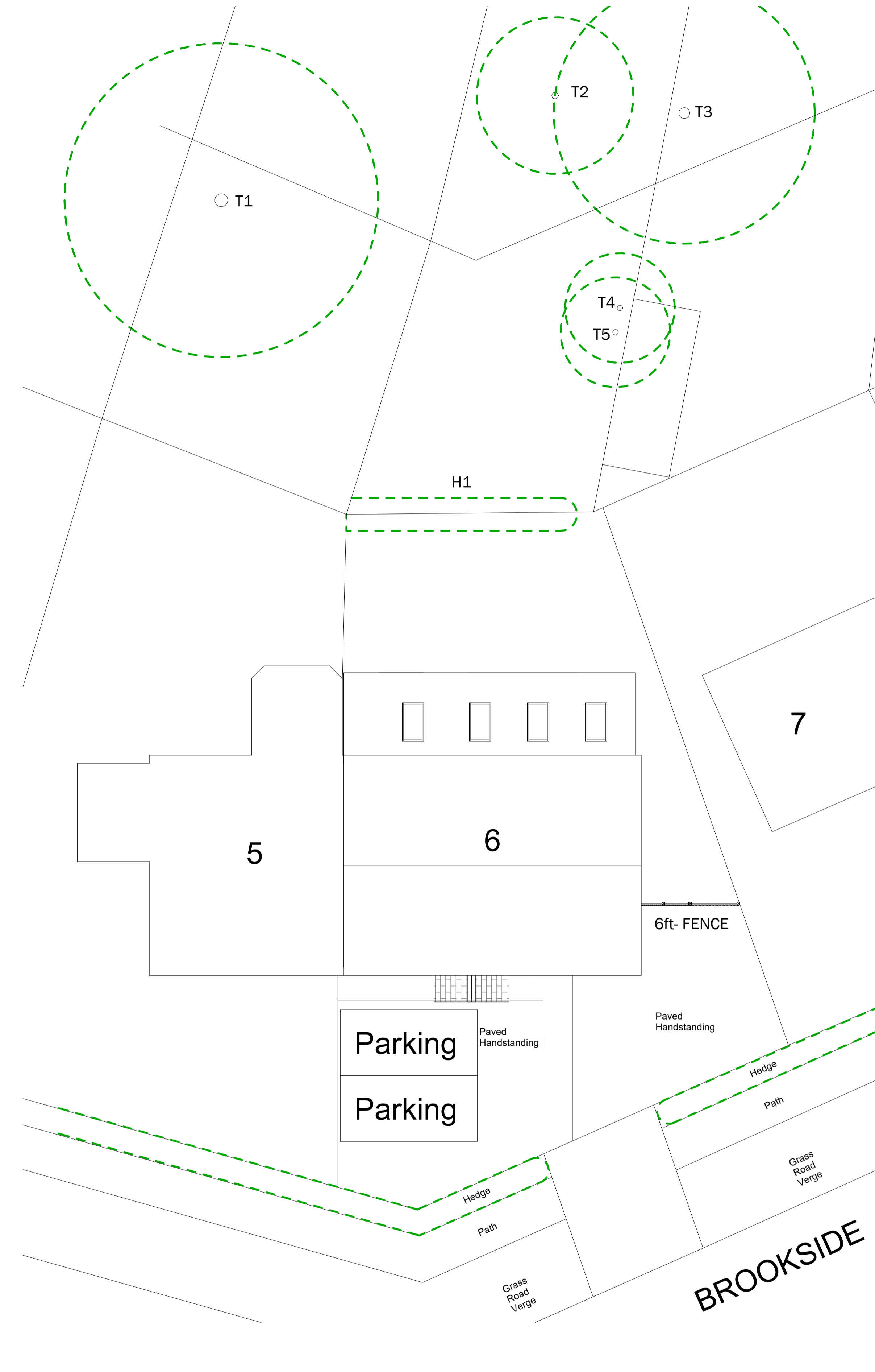
2 PROPOSED SITE PLAN
