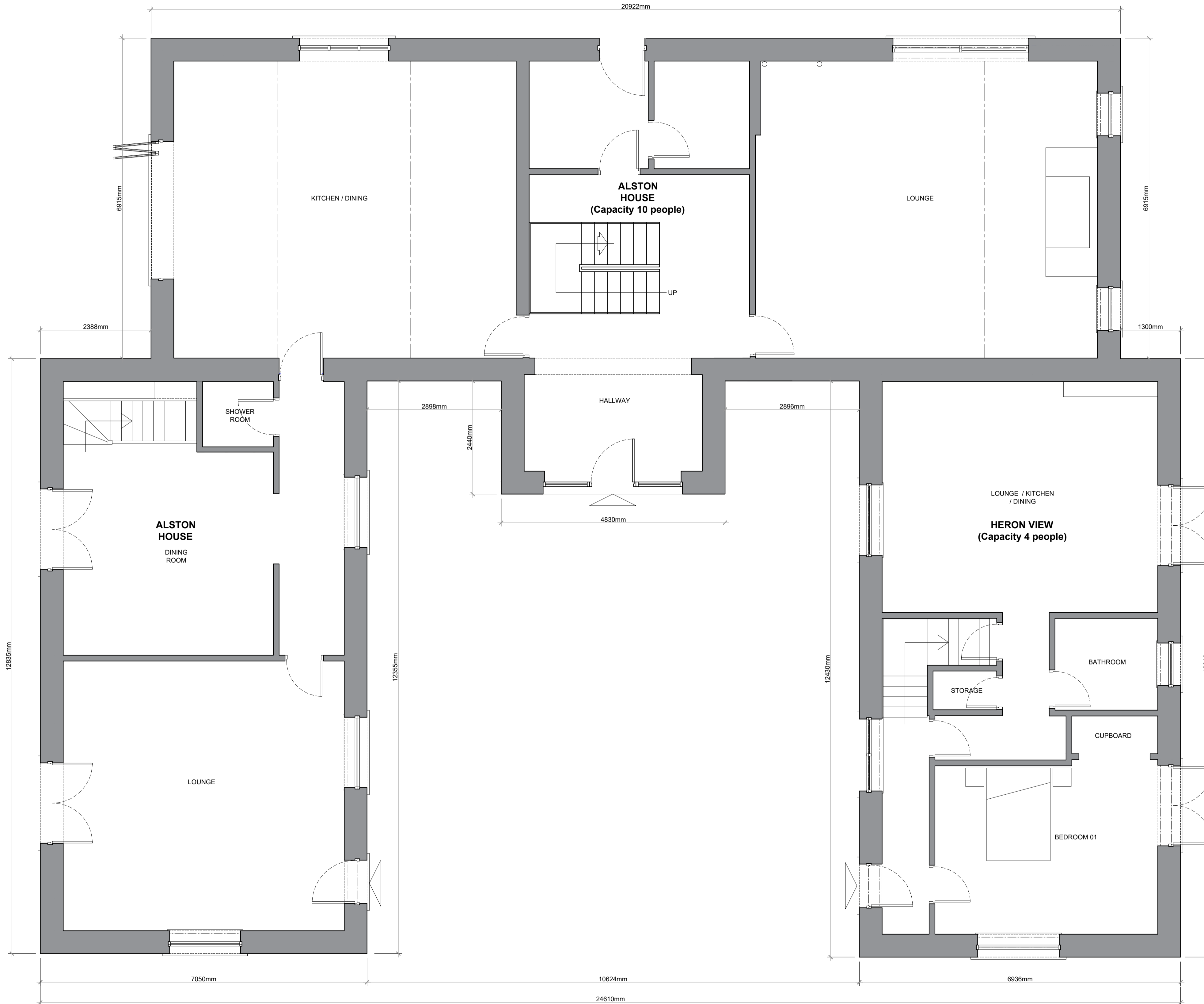
PROPOSED GROUND FLOOR SCALE 1:50
