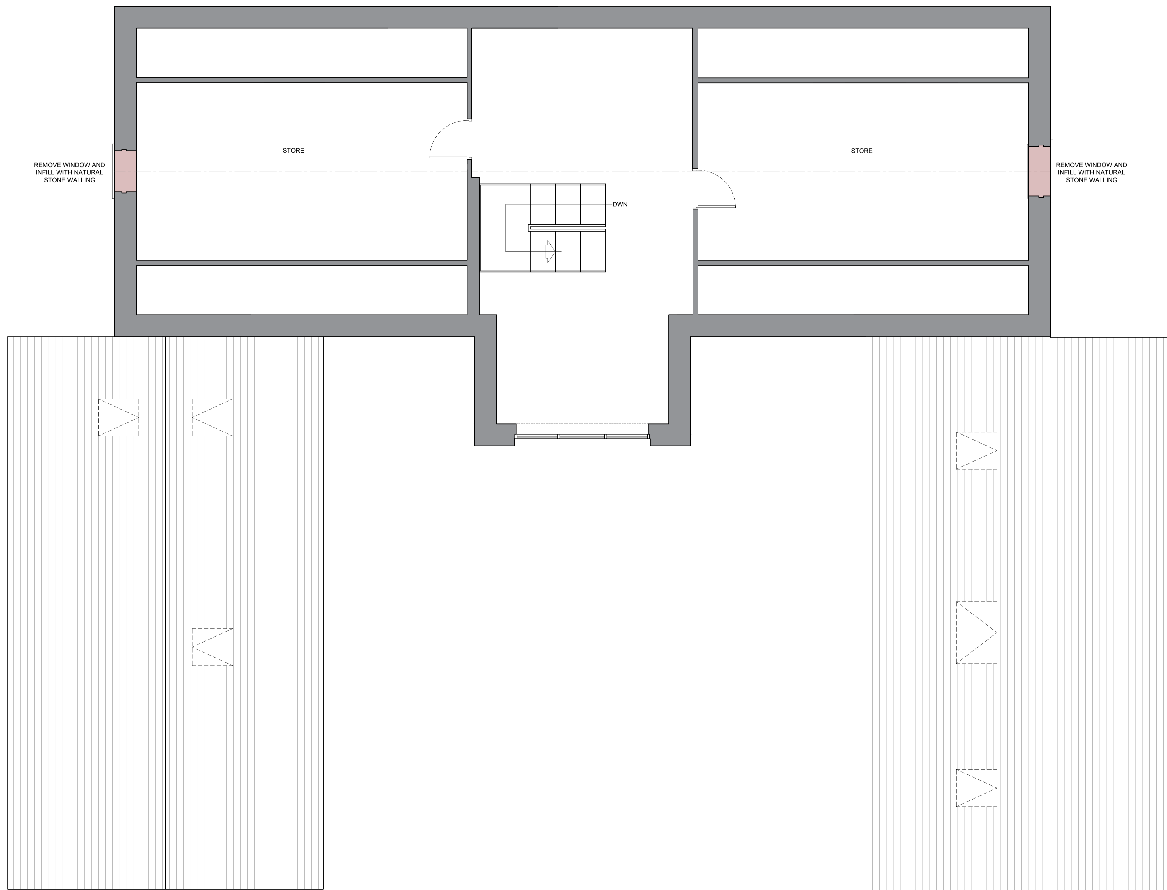
PROPOSED SECOND FLOOR SCALE 1:50
