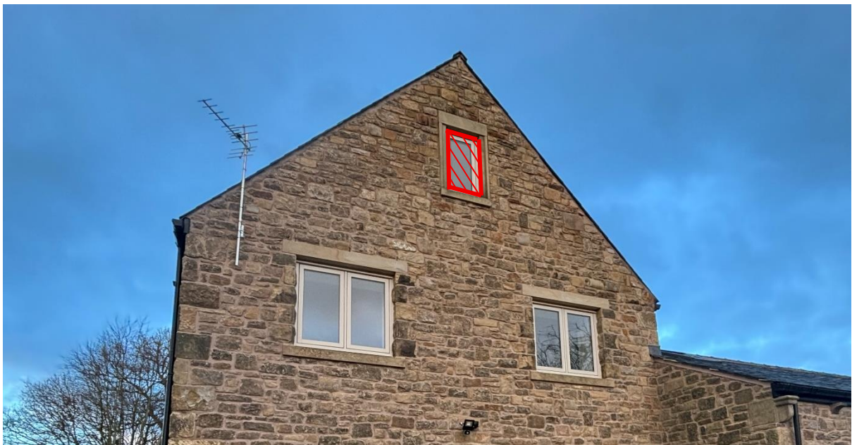
Figure 07– Shows the mortar bedded eave to the South elevation of Alston House main roof (Hatched window to be removed).
