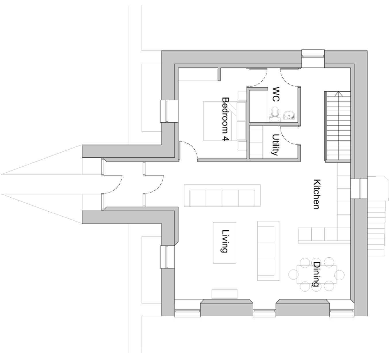
Field Barn Existing Upper Entrance Level Plan
