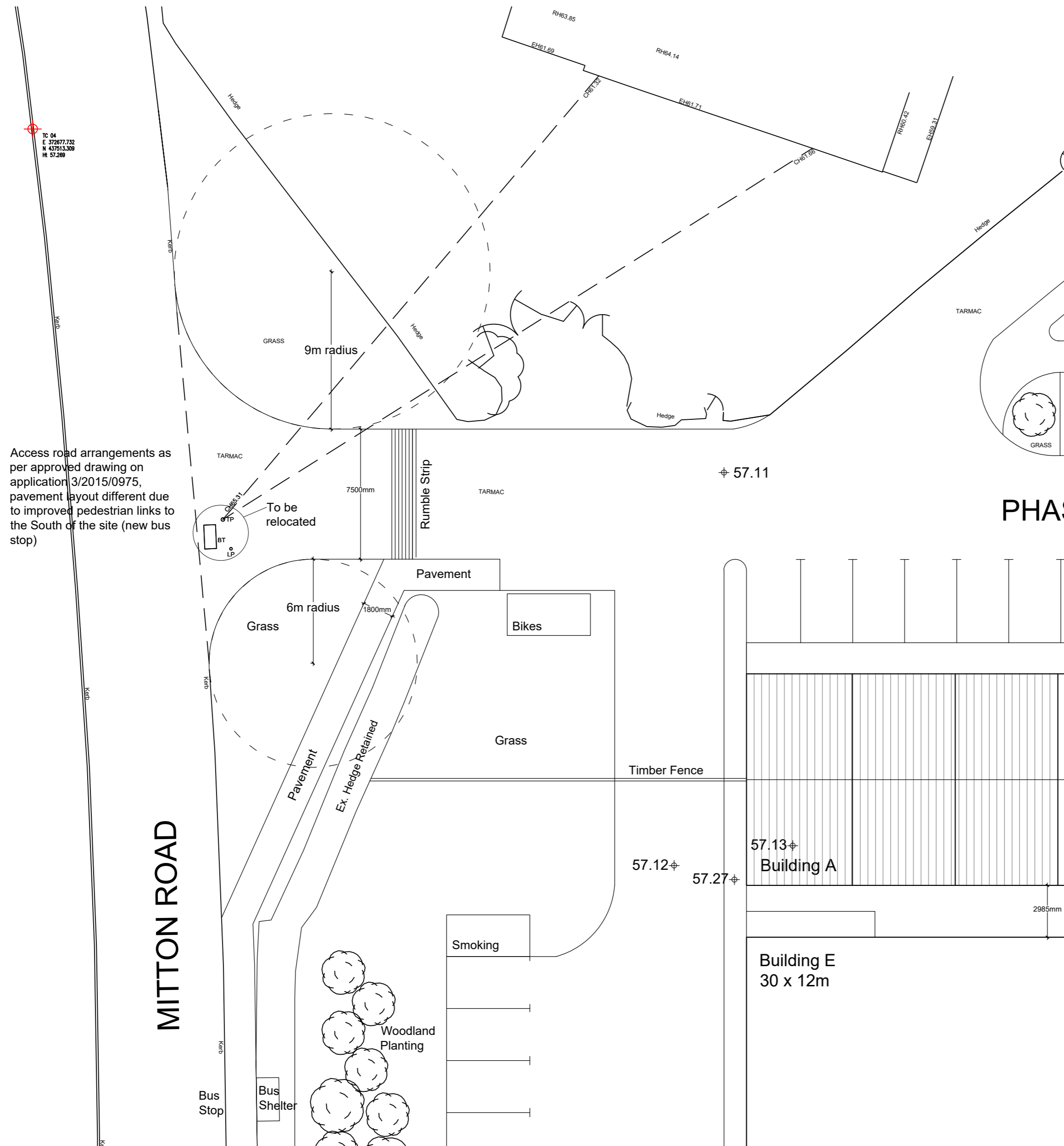
Proposed Site Access 1:200
