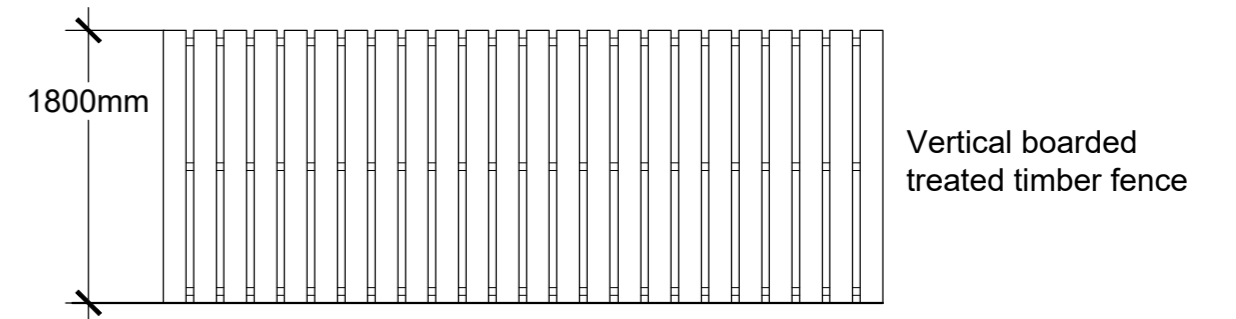
Proposed Fence Detail 1:50
