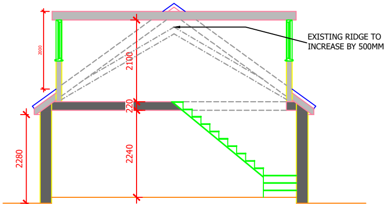
PROPOSED SECTION
