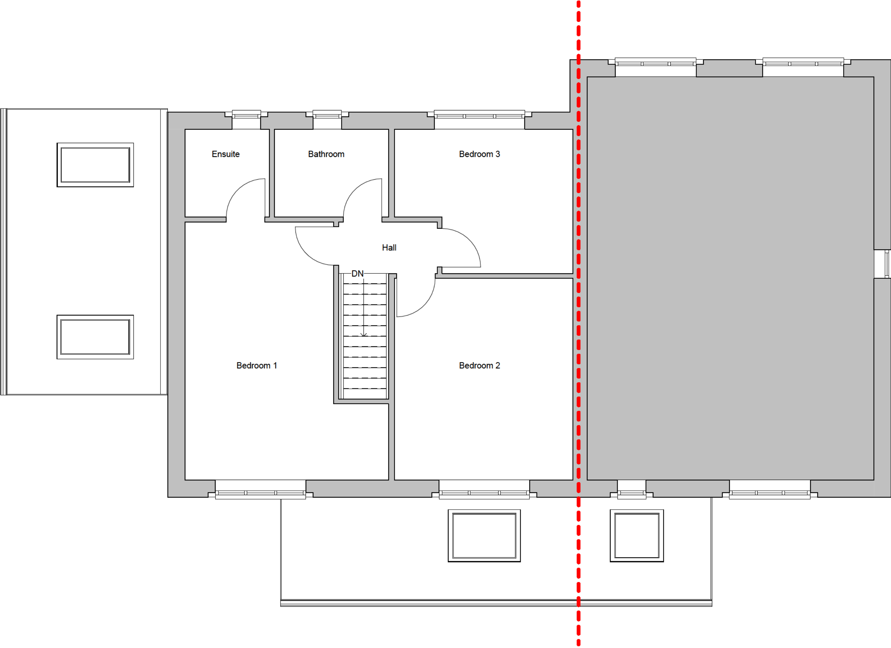
First Floor 1 : 50
