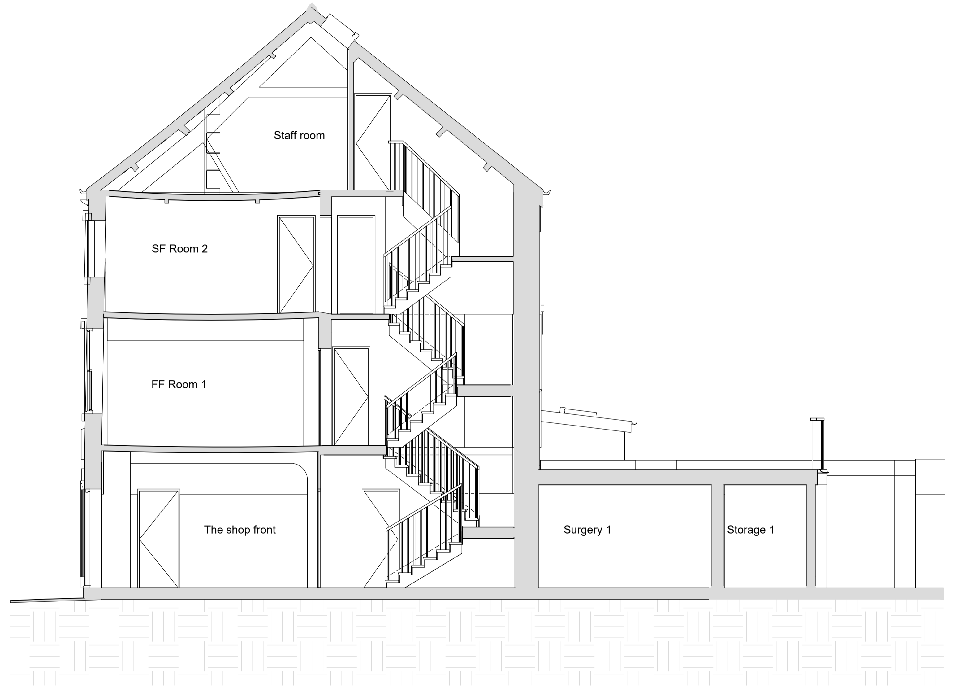
Existing Section B 1:50 Scale
