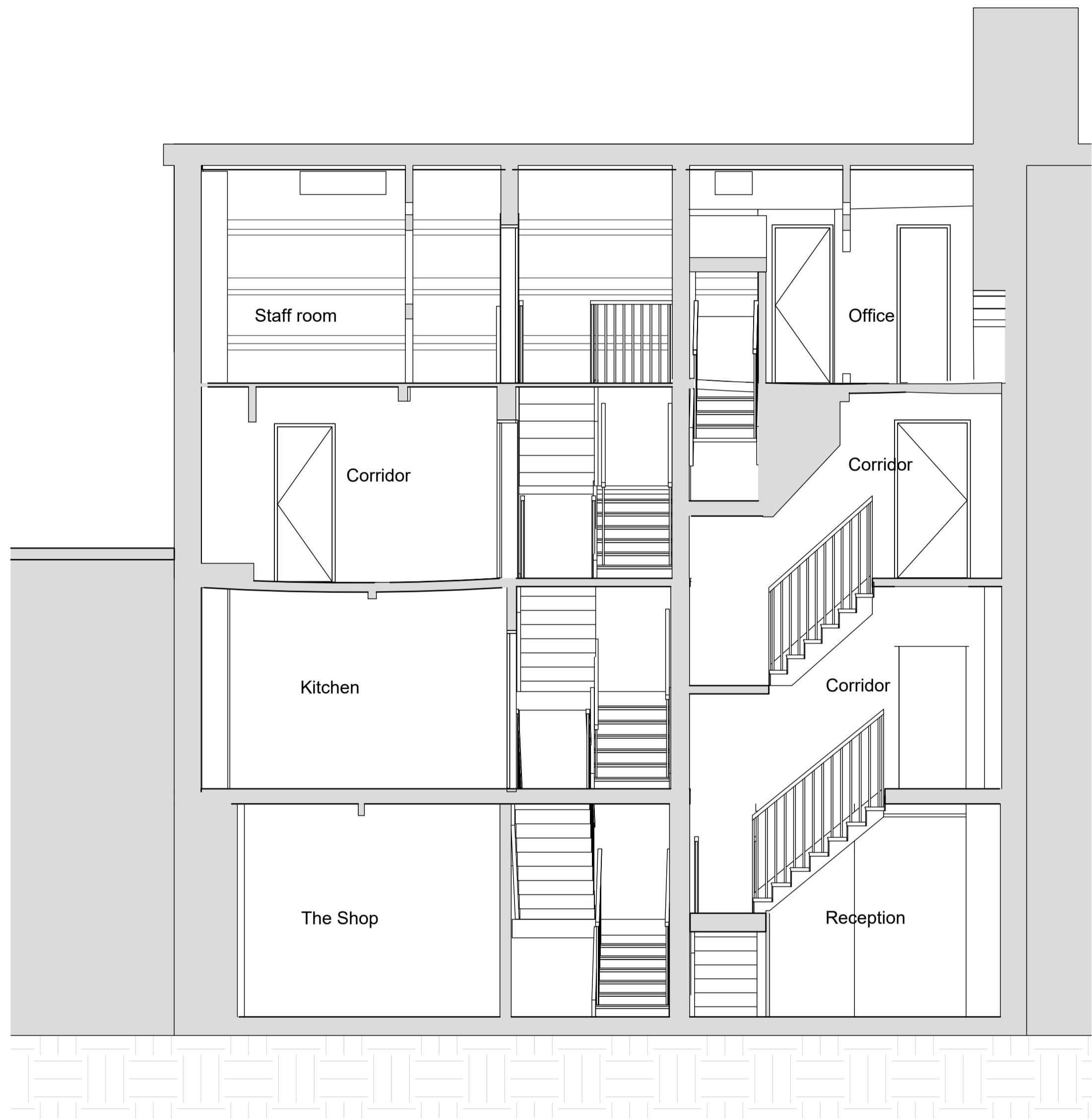
Existing Section A 1:50 Scale
