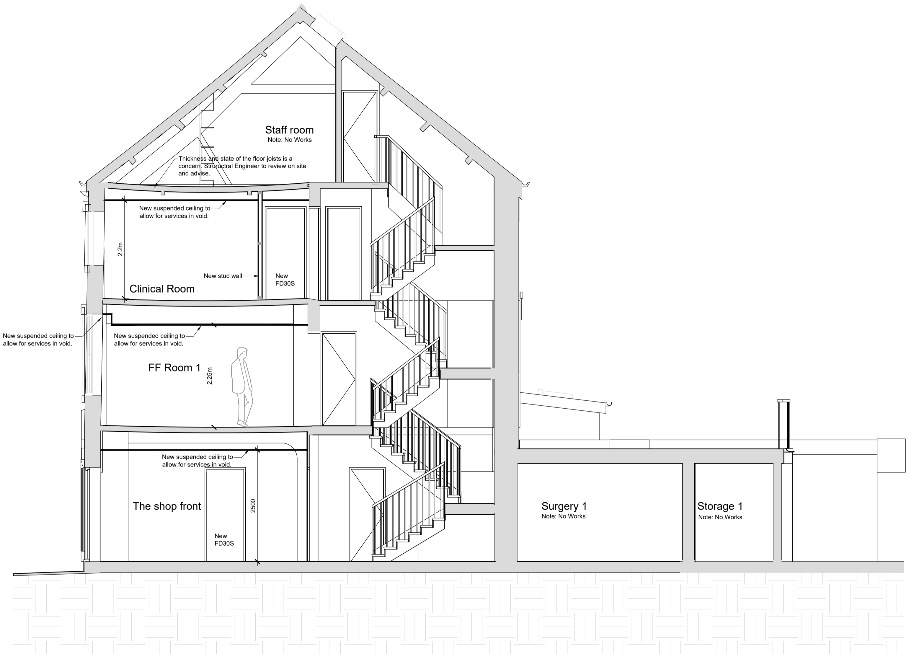
Proposed Section B 1:50 Scale
