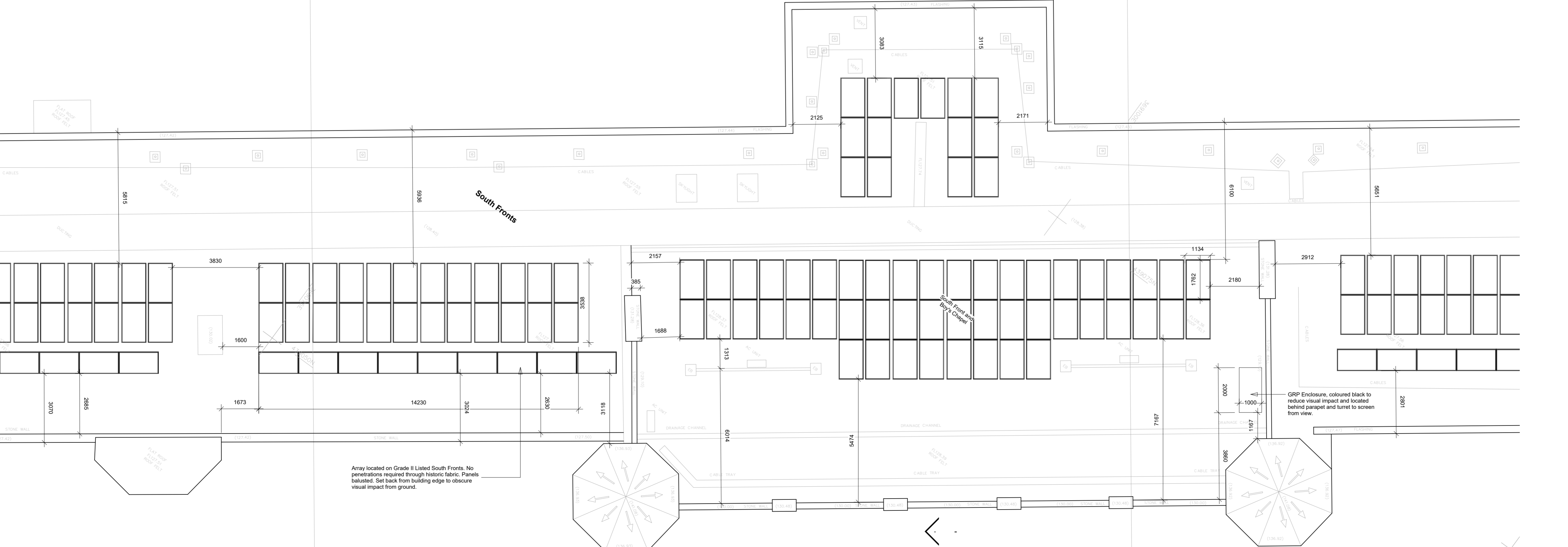
2 | Level 00 South Fronts Mid - Proposed 1:100
