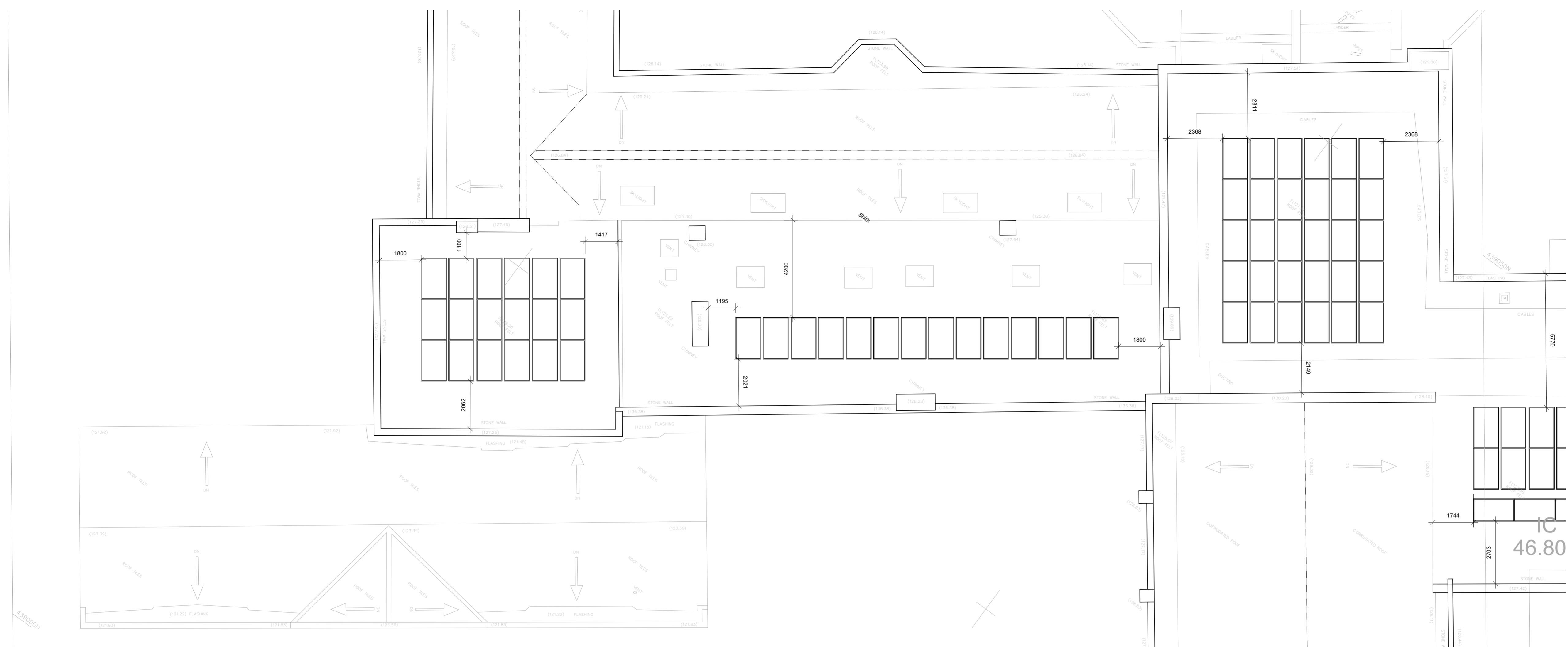
1 | Level 00 South Fronts West - Proposed 1:100
