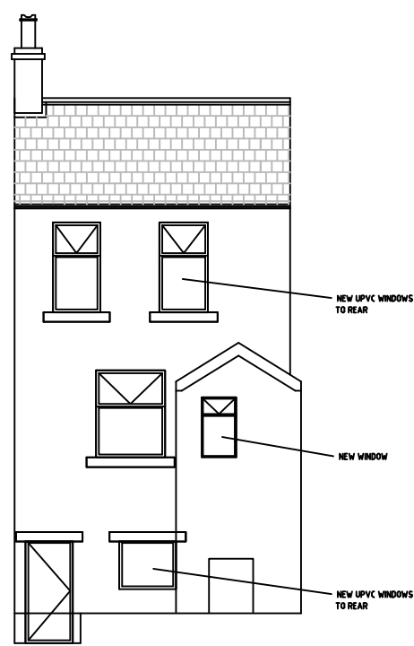
REAR ELEVATION
